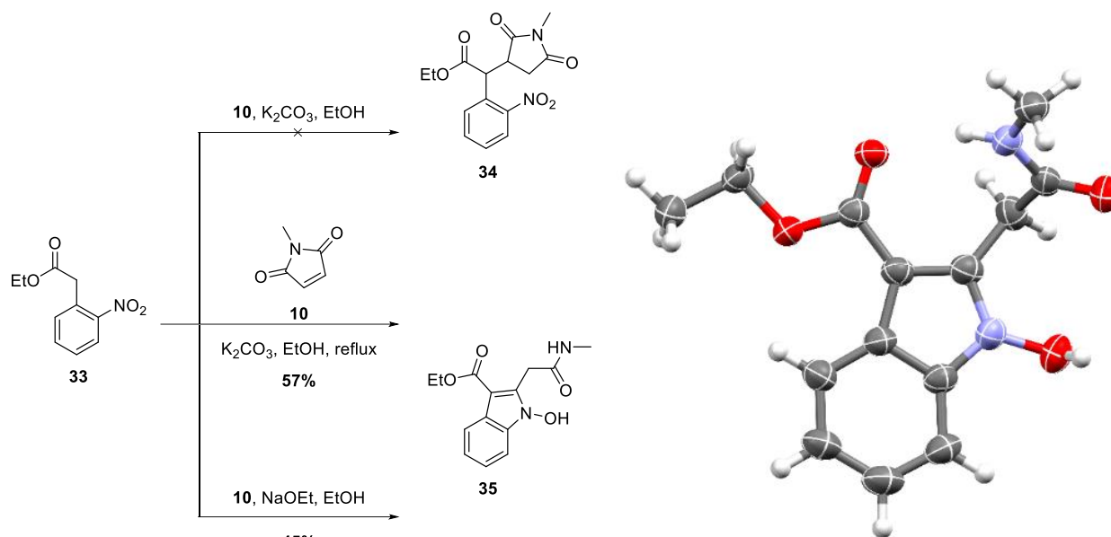
Scheme 6. Annulation reactions of 33 and N -methylmaleimide ( 10 ). The representation of the X-ray crystal structure of N -hydroxyindole 35 has displacement envelopes at 50% probability amplitude, with hydrogen atoms assigned arbitrary radii.
