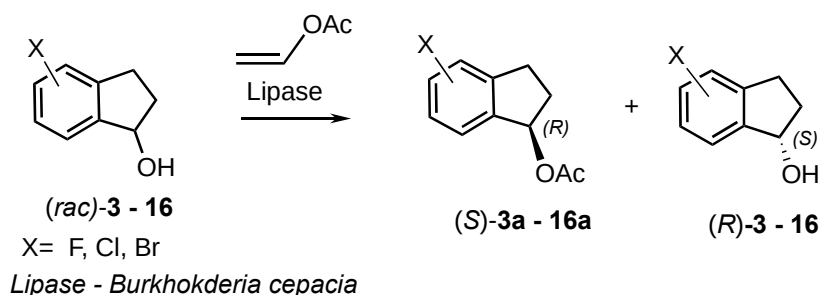
Figure 1. Resolution of racemic halo-2,3-dihydro-1 H -indenols ( rac )-3 - 16 via enzymatic esterification.
