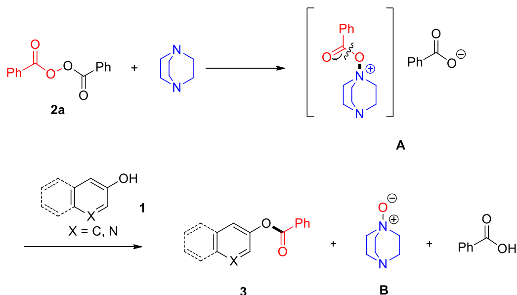
Scheme 3 Plausible mechanism.
