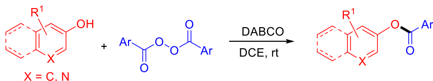
Scheme 1. Methods towards the synthesis of aromatic esters.
