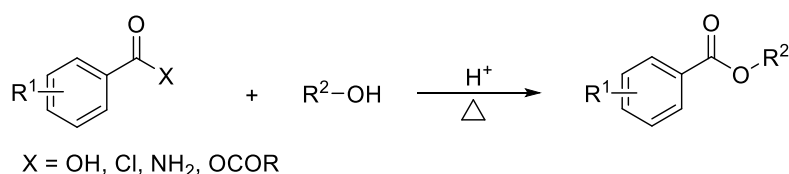
(a) Fischer esterification
