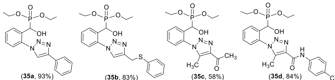
Scheme 29. Sodium carbonate-catalyzed solvent-free synthesis of \alpha -hydroxyphosphonates containing functionalized 1,2,3-triazoles with heating.
