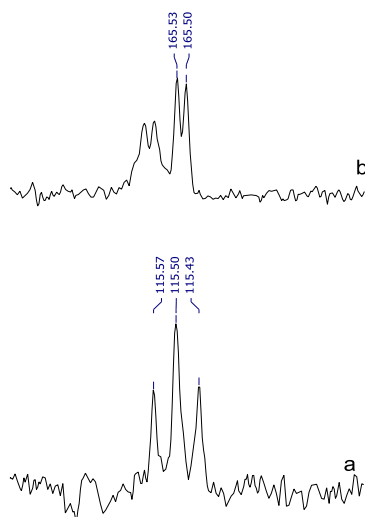
Figure 3. Fragments of ^{13}\text{C} NMR spectra 50 decoupled from ethyl \text{CH}_2 protons (scale is the same): a) CN signal at 115.5 ppm, b) \text{COOEt} signal at 165.5 ppm.
