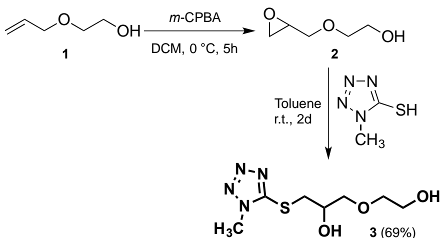
Scheme 1. Synthetic pathway to the 1-(2-hydroxyethoxy)-3-[(1-methyl-1 H -tetrazol-5-yl)thio]propan-2-ol ( 3 ).
