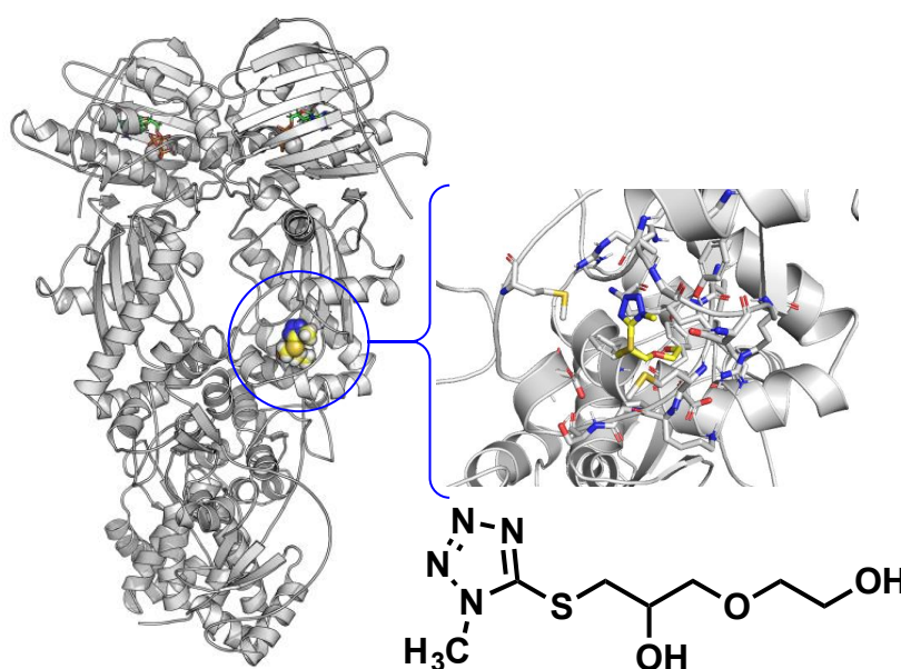
Figure 1. Structure of the 1-(2-hydroxyethoxy)-3-[(1-methyl-1H-tetrazol-5-yl)thio]propan-2-ol and TRAP1 with the tetrazole derivative. TRAP1 monomers are shown in light gray; the ligand is depicted with C atoms in yellow. The inset shows the details of interactions in the complex.
