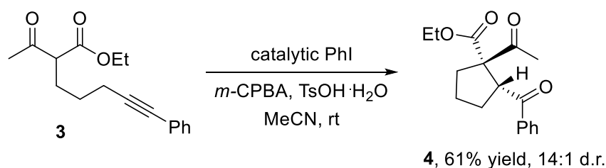
(b) This work: alkyne activation?
