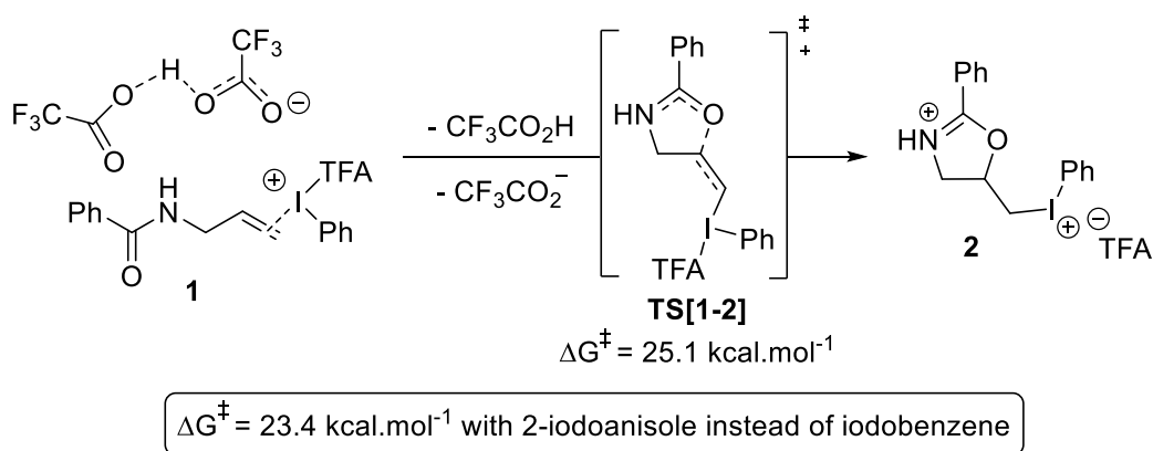
(a) Previous work: alkene activation
