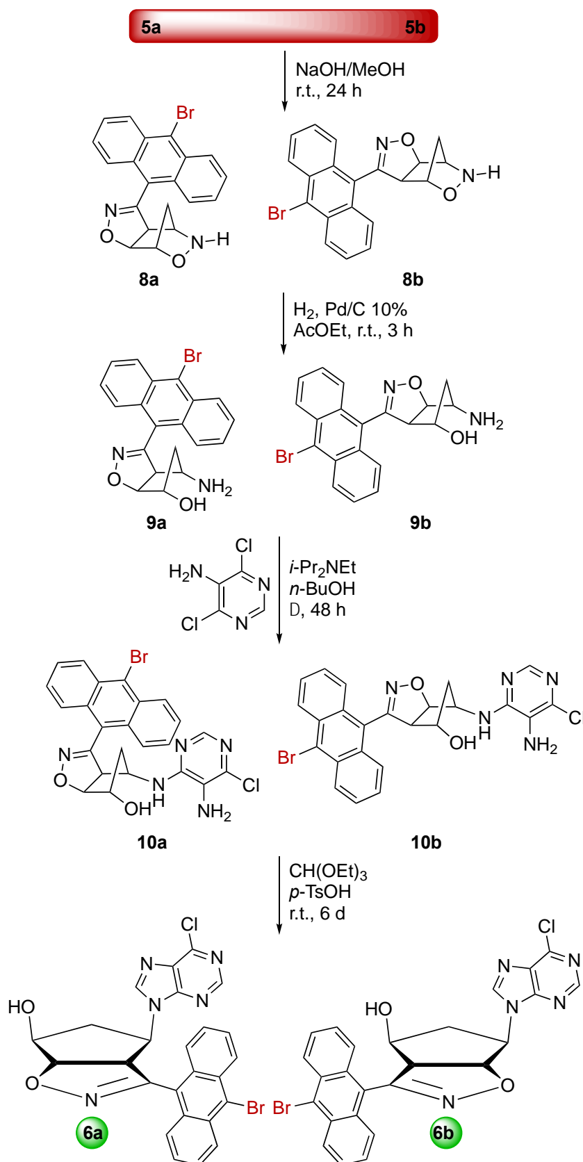
Scheme 3. Synthetic pathway to brominated regioisomeric nor-nucleosides 6a,b .
