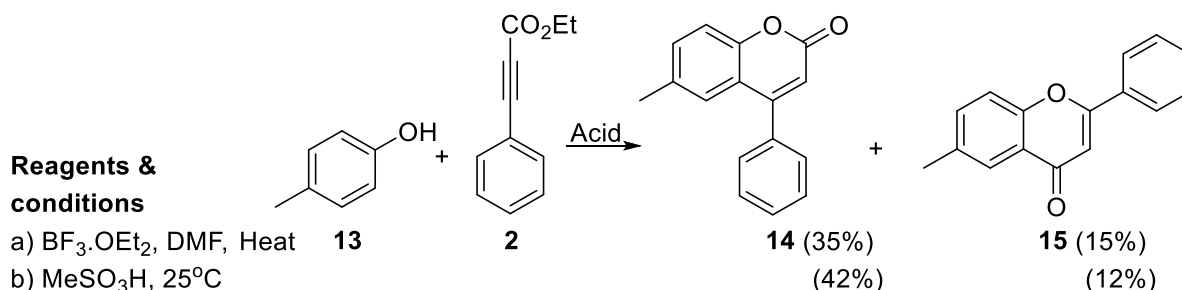
Scheme 5. Acid-mediated reaction of p -cresol and propiolate 2 .
