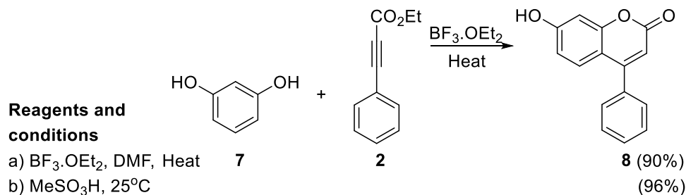
Scheme 3. Acid-mediated reaction of resorcinol 7 and propiolate 2 .
