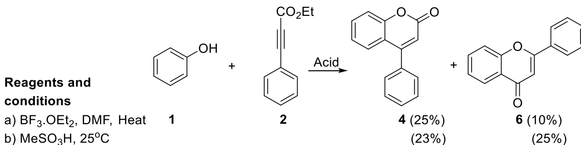
Scheme 2. Acid-mediated reaction of phenol 1 and propiolate 2 .
