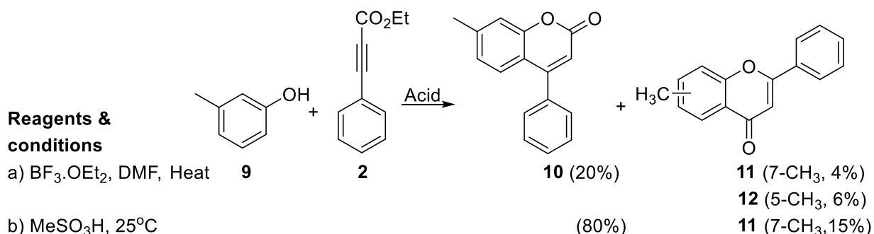
Scheme 4. Acid-mediated reaction of m -cresol and propiolate 2 .
