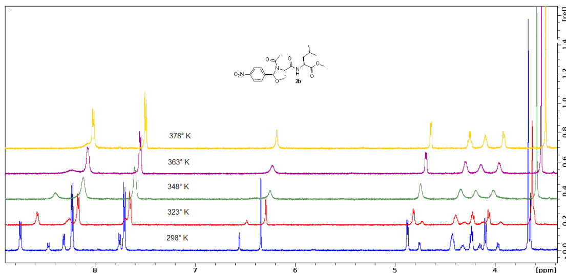
Figure 2. ^1\text{H} NMR spectra of compound 2b in \text{DMSO-d}_6 at different temperatures (3.5-9 ppm).
