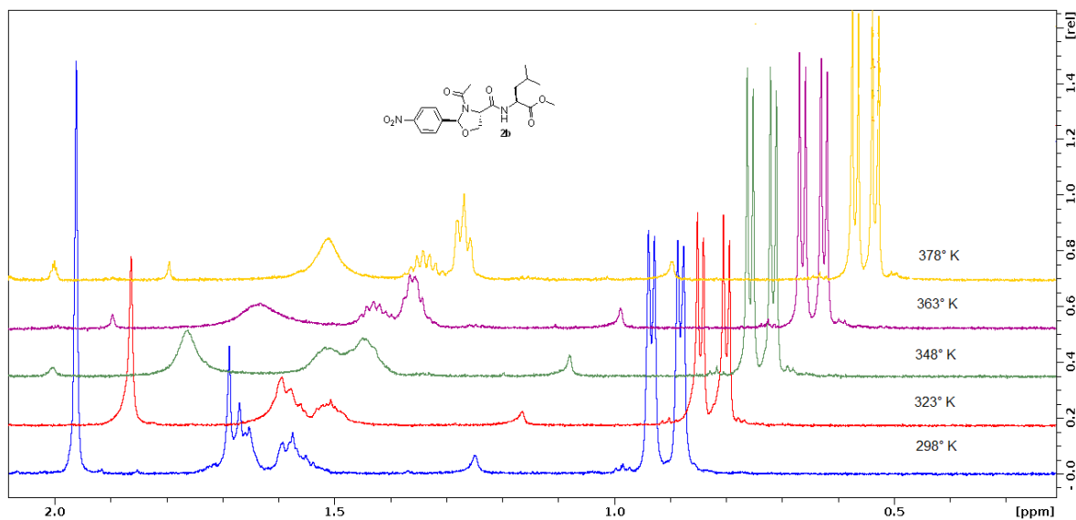
Figure 3. ^1\text{H} NMR spectra of compound 2b in \text{DMSO-d}_6 at different temperatures (0-2ppm).
