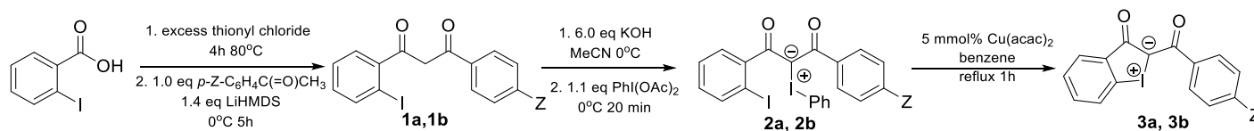
Scheme 1. Synthesis of cyclic iodonium ylide compounds. (a: Z=H, b: Z=NO 2 )
