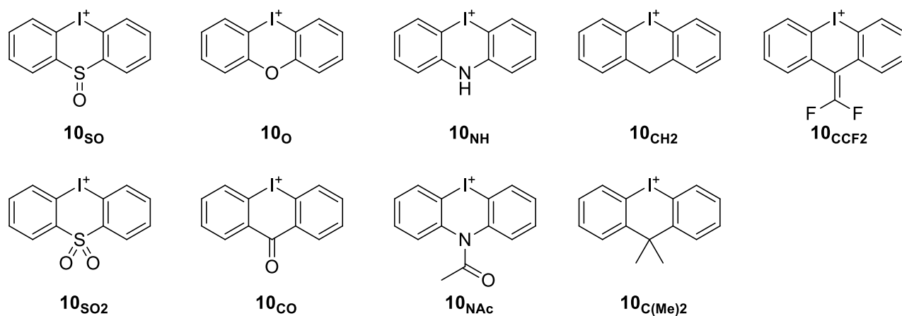
Figure 9. Iodonium cations considered in this work.
