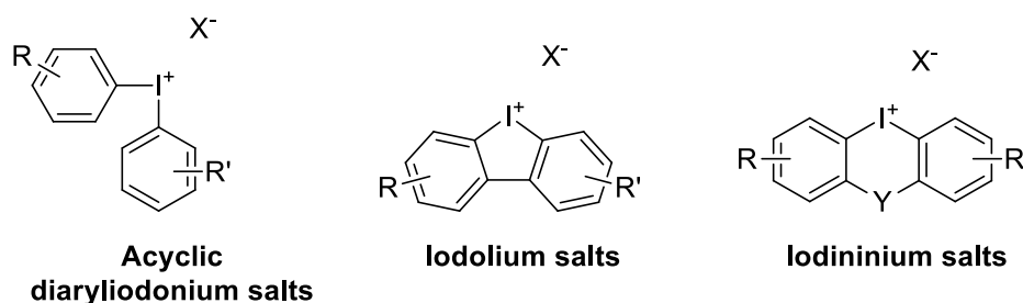
Figure 1. Classes of iodine(III) halogen bond donors.
