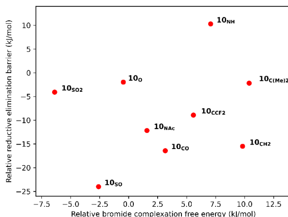
Figure 10. Relative reductive elimination barrier and bromide complexation free energy of iodonium cations 10 compared to the unfunctionalized iodonium cation 1 H .
