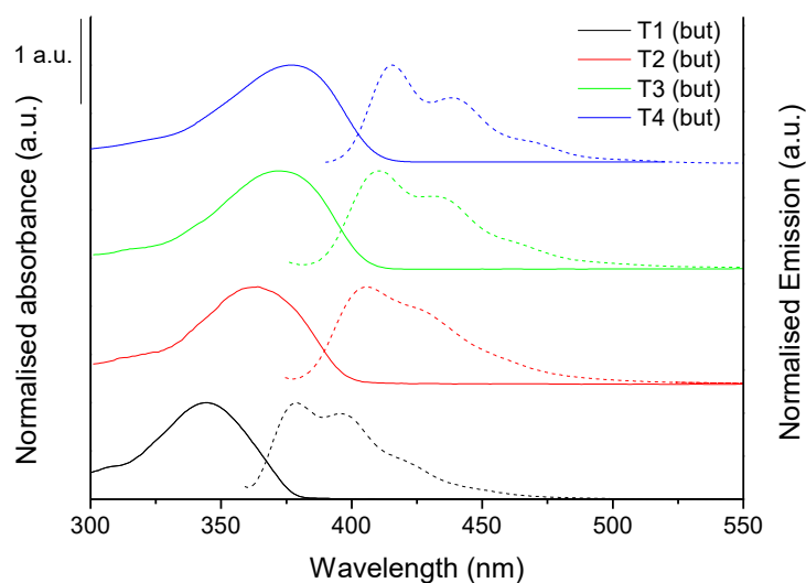
Figure 9. Normalized absorption (continuous line) and emission (dashed line) spectra of the members of the Tn (butyl) family ( 10^{-6} M solutions in 1:2 acetonitrile:benzene).
