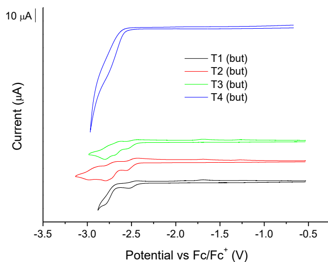
Figure 6. Reduction waves of the Tn (butyl) series in 1:2 acetonitrile:benzene. The cyclic voltammogram was obtained employing a glassy carbon working electrode, a platinum wire counter electrode and a silver wire reference electrode. All the waves were referenced to ferrocene.
