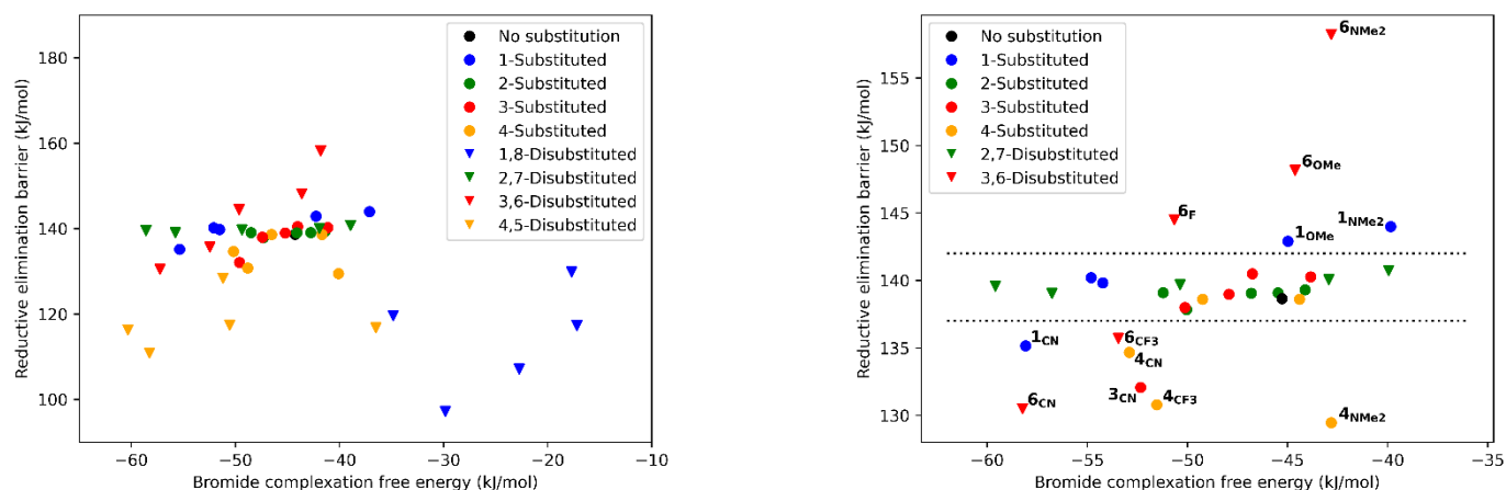
Figure 3. a) Relationship between the reductive elimination barrier and the Lewis acidity; b) Same relationship but excluding 1,8-disubstituted and 4,5-disubstituted compounds.
