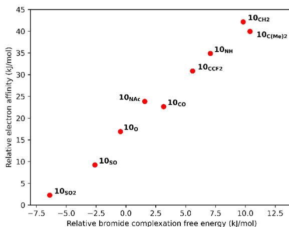
Figure 12. Relative vertical electron affinity and bromide complexation free energy of iodinium cations compared to the unfunctionalized iodonium cation 1 H .
