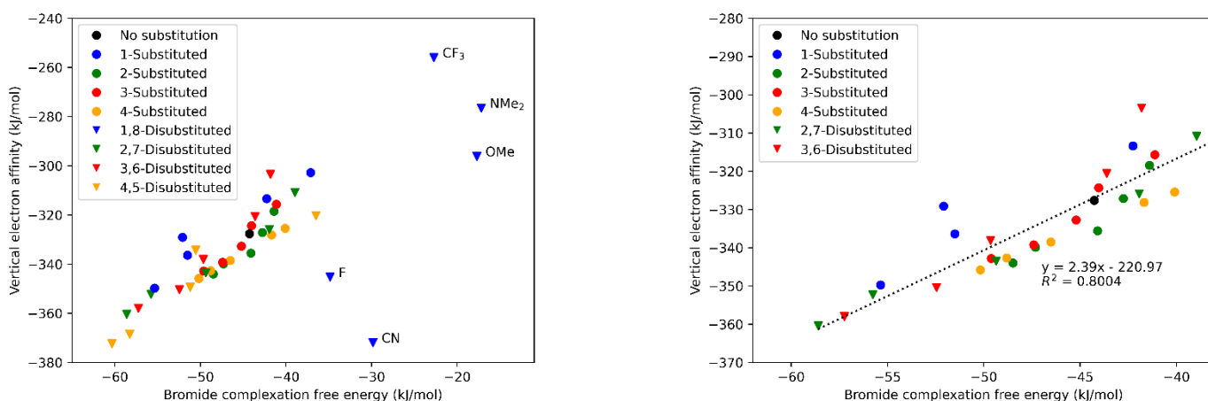
Figure 7. a) Variation of the vertical electron affinity of iodolium cations; b) Same trend, but without 1,8-disubstituted and 4,5-disubstituted compounds.
