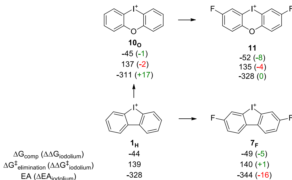
Figure 13. Comparison of fluorinated iodonium and iodinium cations.
