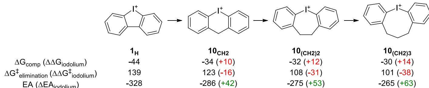
Figure 14. Comparison of cyclic diaryliodonium compounds bridged by an alkane chain of different lengths.
