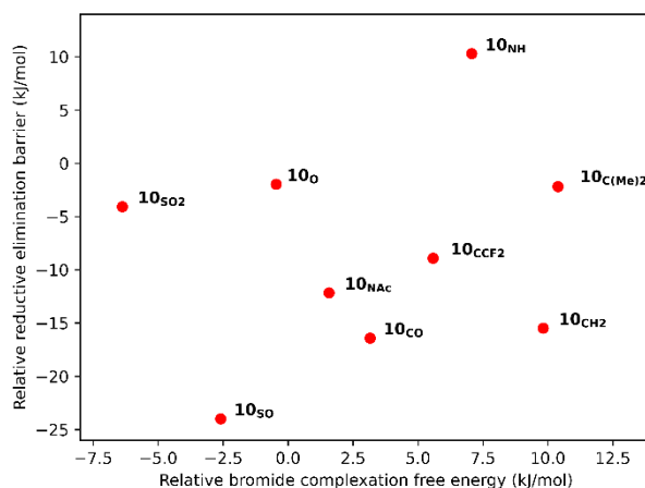
Figure 10. Relative reductive elimination barrier and bromide complexation free energy of iodinium cations 10 compared to the unfunctionalized iodolium cation 1 H .
