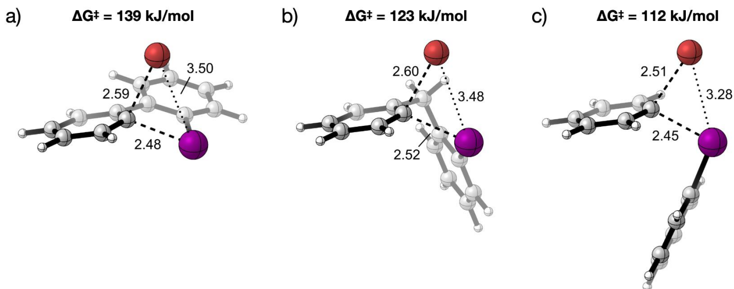
Figure 11. Reductive elimination transition states of: a) iodolium bromide; b) iodinium (methylene bridged) bromide; c) diphenyliodonium bromide.
