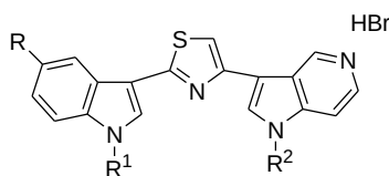
Indolyl-thiazolyl-5-azaindoles
