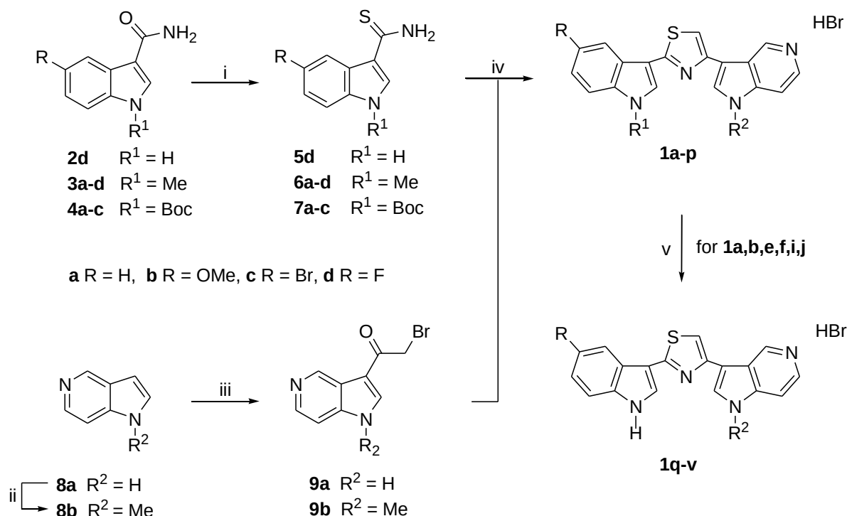
Scheme 1. Synthesis of indolyl-5-azaindolyl thiazole hydrobromides 1a-v . Reagents and conditions: (i) Lawesson's reagent, toluene or benzene, reflux, 0.5-24 h, 90-98%; (ii) t -BuOK, toluene, TDA-1, rt, 4 h; then MeI, rt, 16 h, 60%; (iii) AlCl_3 , DCM, BrCOCH_2Br , reflux, 40 min (for derivative 9a ) or 15 min (for derivative 9b ), 90-93%; (iv) EtOH, reflux, 1 h, 58-84%; (v) TFA, DCM, reflux, 24 h, 62-93%.
