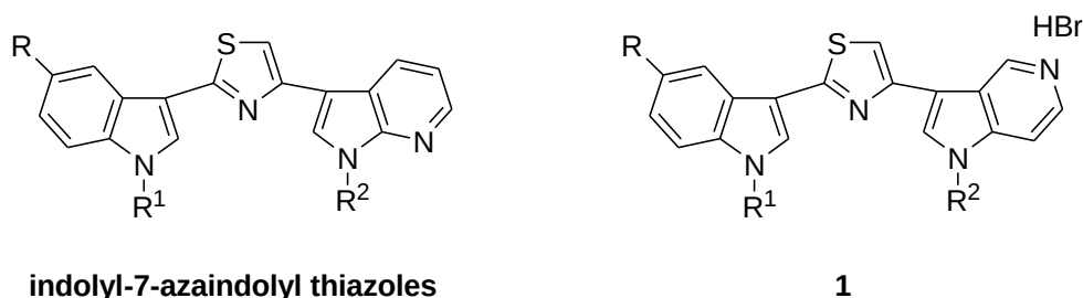
Figure 2. Azaindole derivatives of thiazole nortopsentin analogues.
