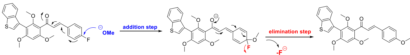
Scheme 3. \text{S}_{\text{N}}\text{Ar} reaction mechanism.
