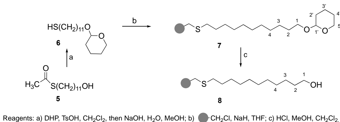
Figure 2. The synthesis of function-bearing polymer bead 8 from reactant 5 .
