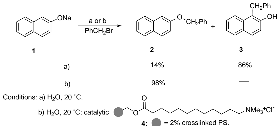
Figure 1. Heterogeneous phase transfer catalysis in water.
