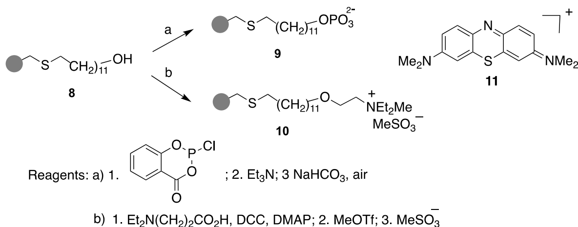
Figure 5. The synthesis of polymer beads for the study of inter-bead ion pairing.
