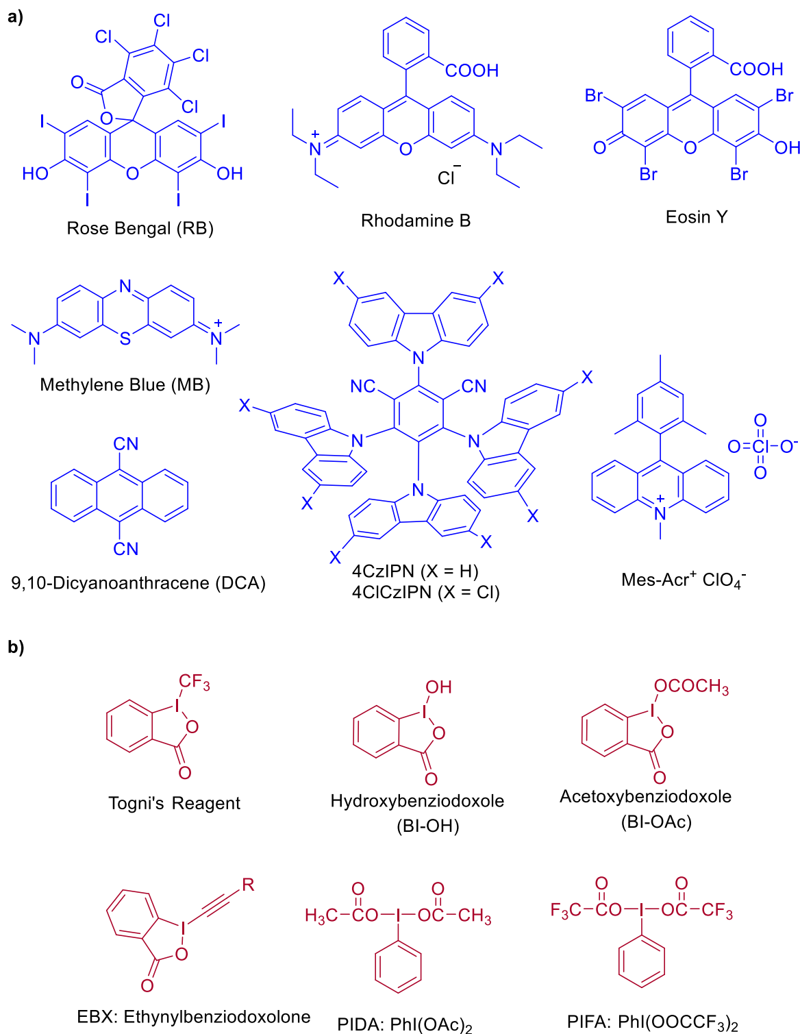
Figure 1. a) Examples of commonly used: a) organo photocatalyst (OPC) and b) hypervalent iodine reagents (HIRs).
