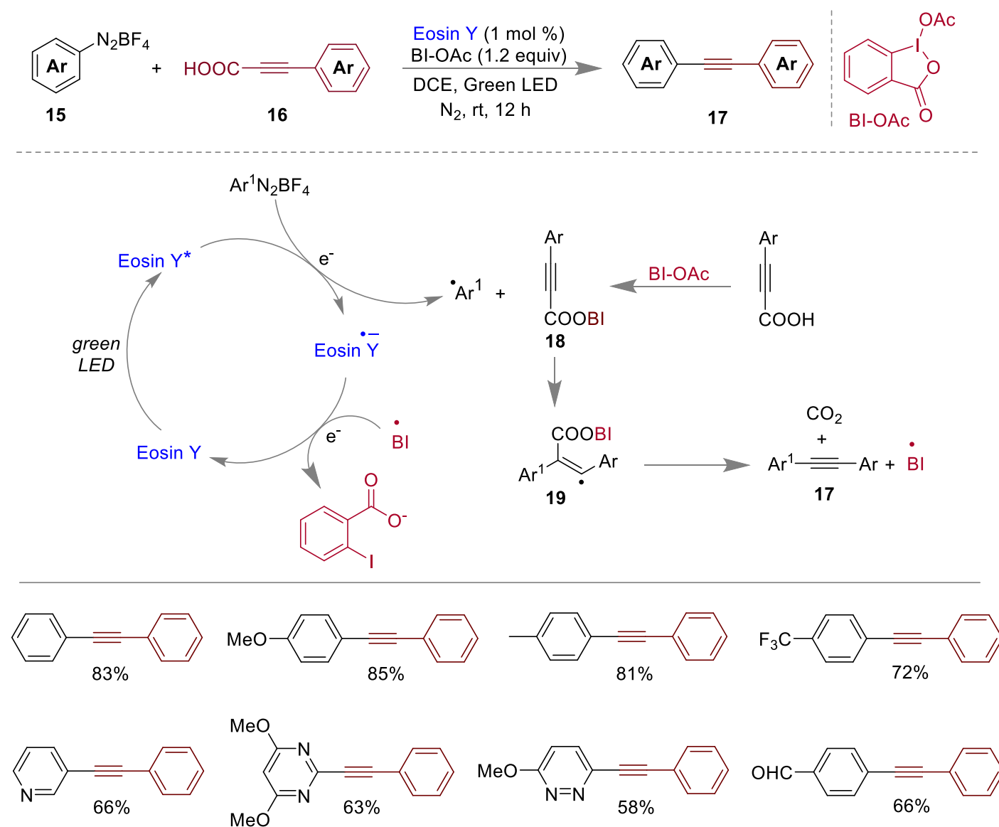
Figure 7. Decarboxylative alkylation of arene diazonium salt using Eosin Y and BI-OAc. 68
