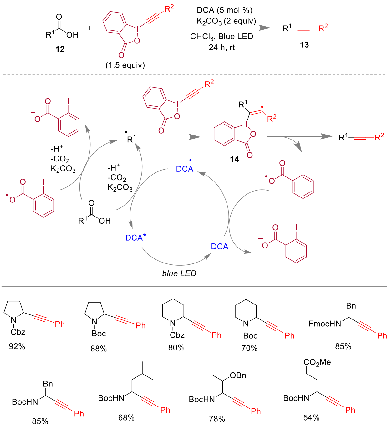
Figure 6. Decarboxylative alkylation using DCA and EBX. 52
