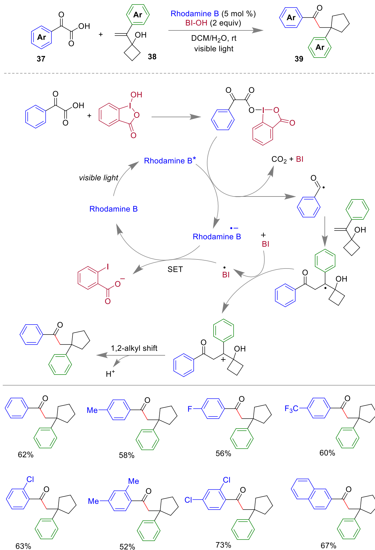
Figure 14. Ring expansion of cyclobutane system using Rhodamine B and BI-OH. 80
