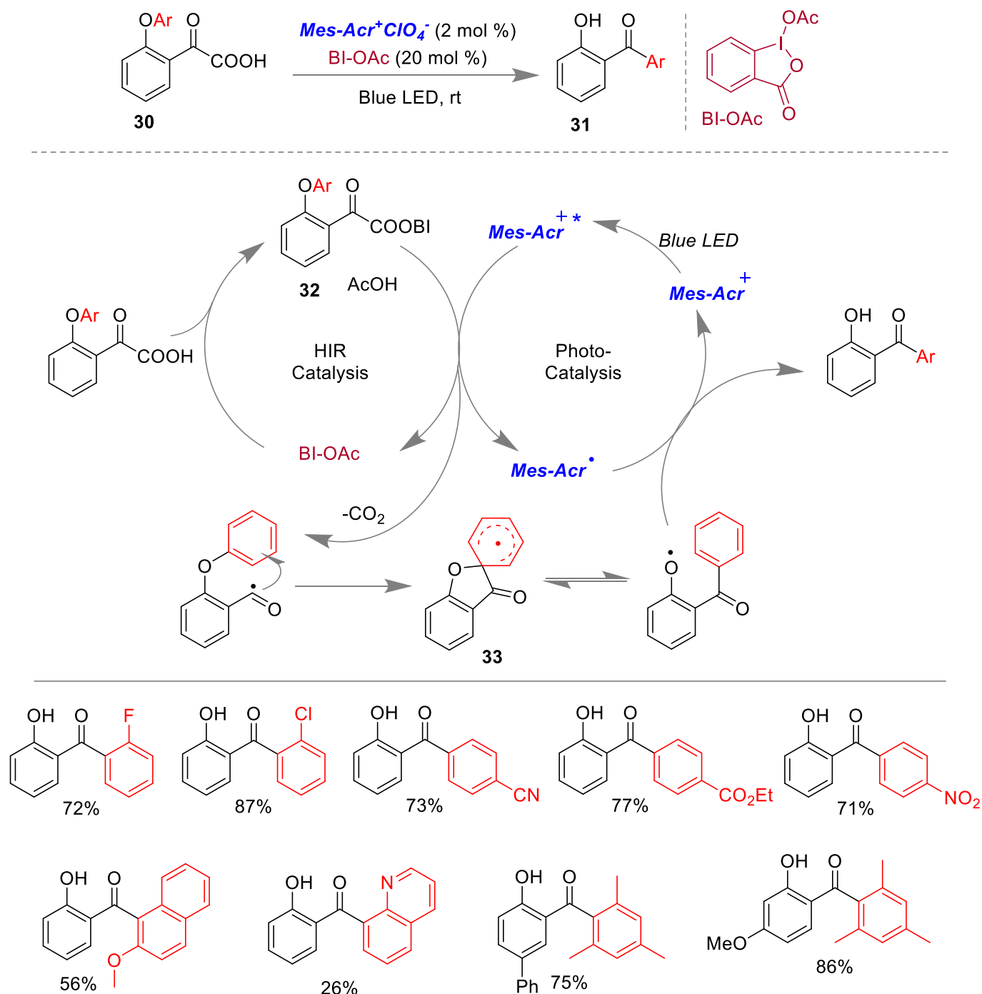
Figure 12. Photo-catalytic Smiles rearrangement using \text{Mes-Acr}^+\text{ClO}_4^- and \text{BI-OAc} . 77
