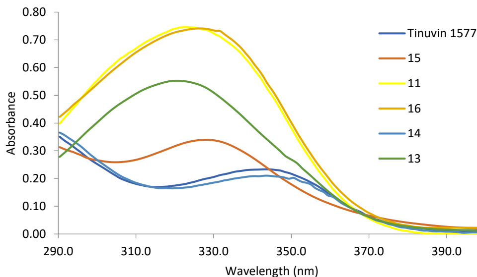
Figure 6. UV absorbance spectra of 0.1 mM solutions of Tinuvin 1577 ( \text{CHCl}_3 ), 11 ( \text{CHCl}_3 ), 13 (DMSO), 14 (DMSO), 15 (DMSO) and 16 (DMSO)
