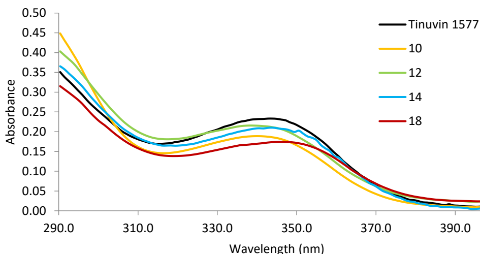
Figure 5. UV absorbance spectra of 0.1 mM solutions of UVAMs 10 (DMSO), 12 (DMSO), 14 (DMSO), 18 (DMSO) and Tinuvin 1577 ( \text{CHCl}_3 )
