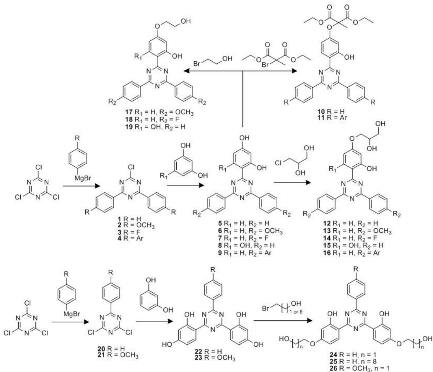
Figure 4. Synthetic routes to UVAMs 10-19 and 24-26
