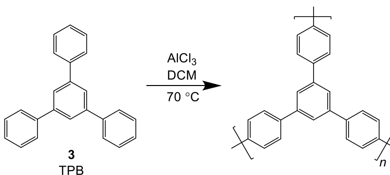
Scheme 2. Synthesis of TPB network polymer.
