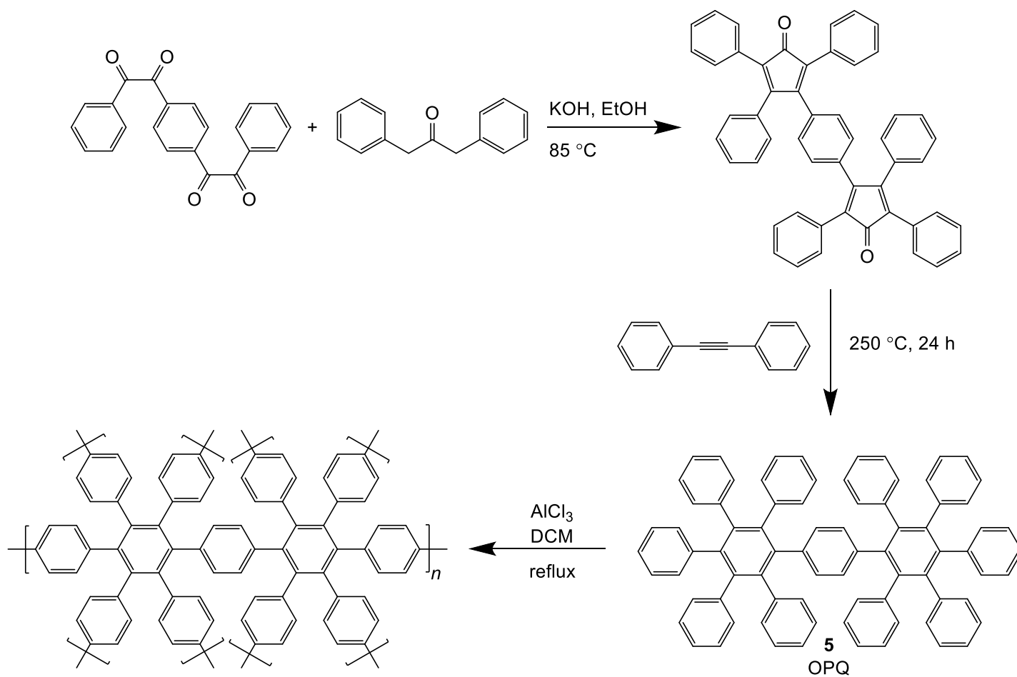
Scheme 4. Synthesis of OPQ network polymer.
