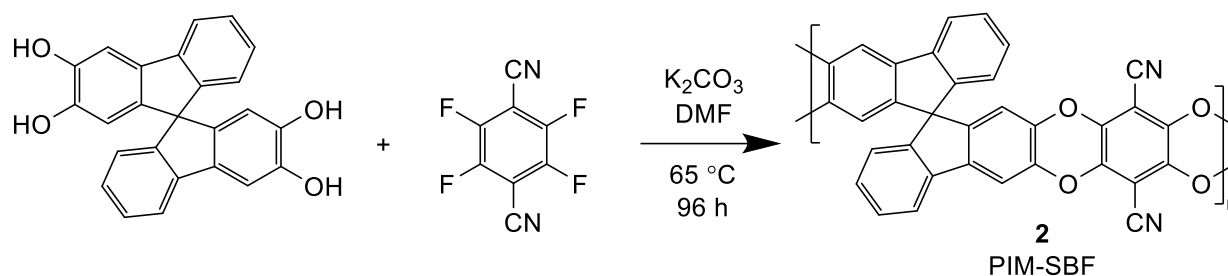
Scheme 1. Synthesis of PIM-SBF.
