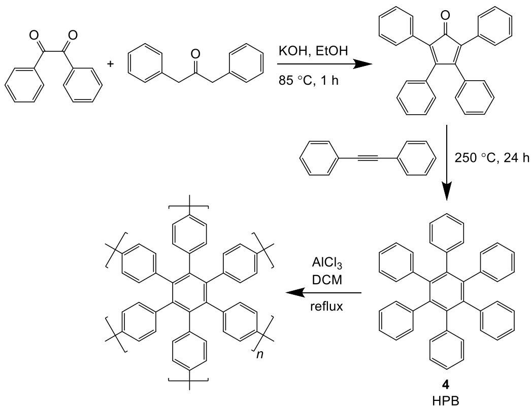
Scheme 3. Synthesis of HPB network polymer.
