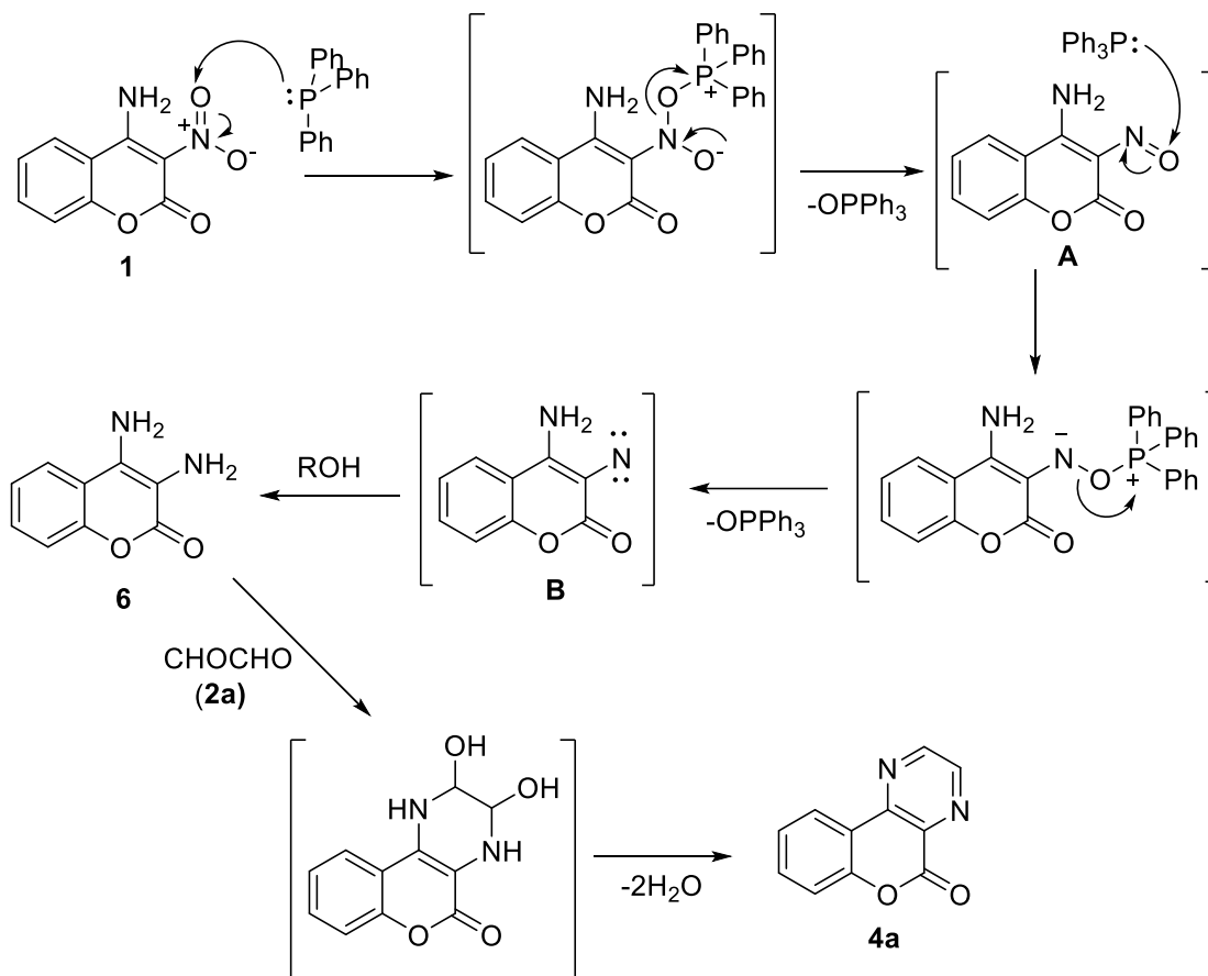
Scheme 2. Proposed mechanism for the one-pot reaction of 1 with 2a in the presence of PPh 3 .
