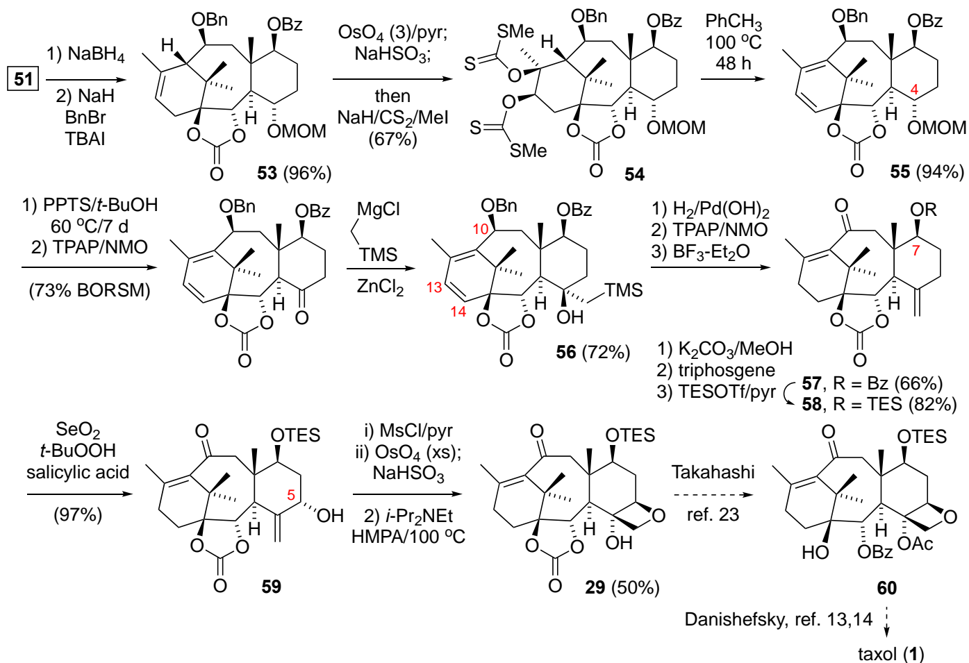
Scheme 10. Final steps of the Chida formal synthesis.
