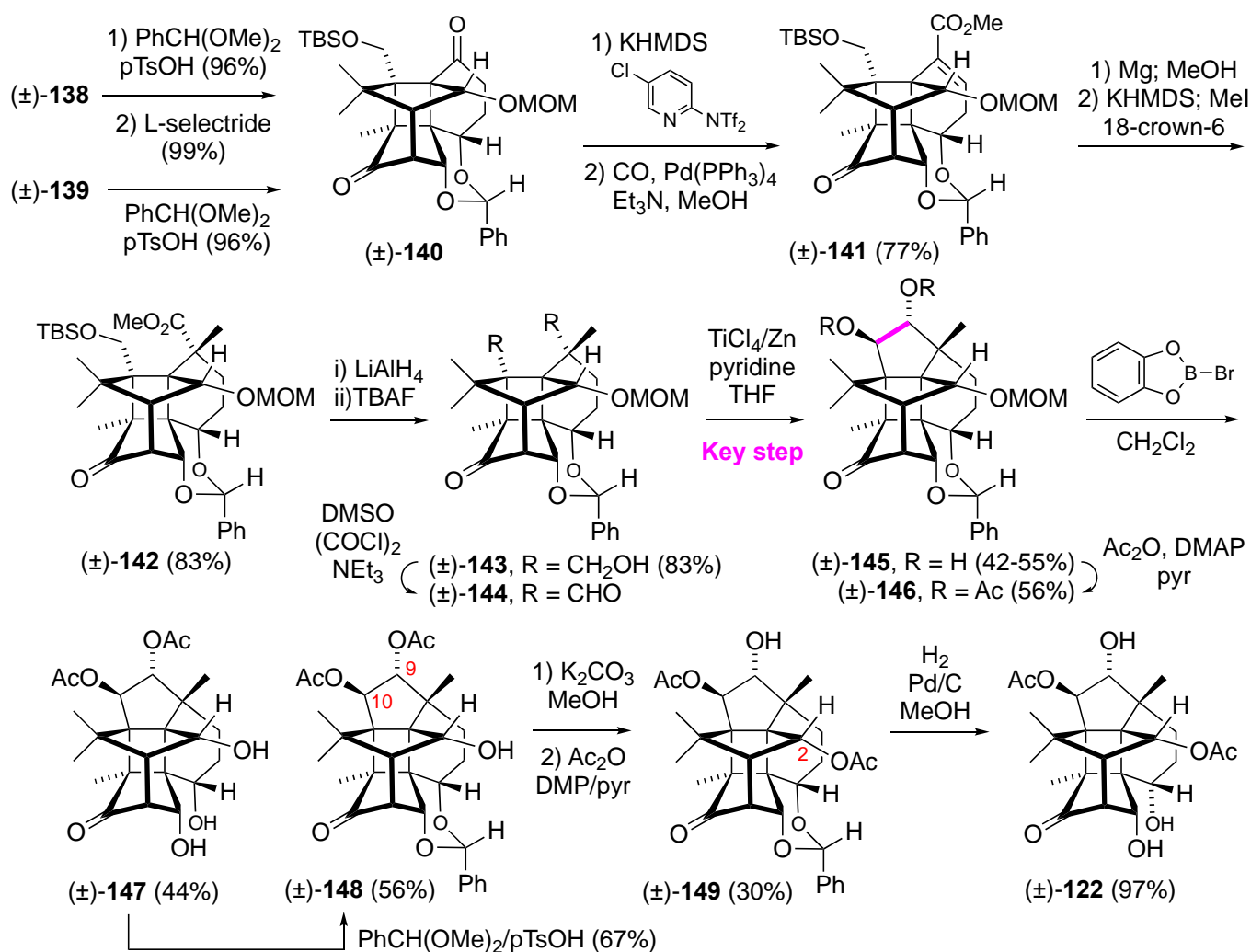
Scheme 23. Completion of the synthesis of rac -cantaxpropellane
