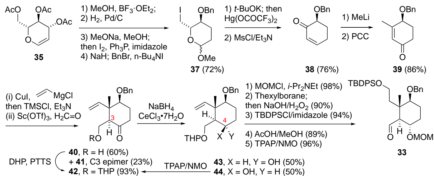
Scheme 8. Synthesis of the ring C fragment 33 .
