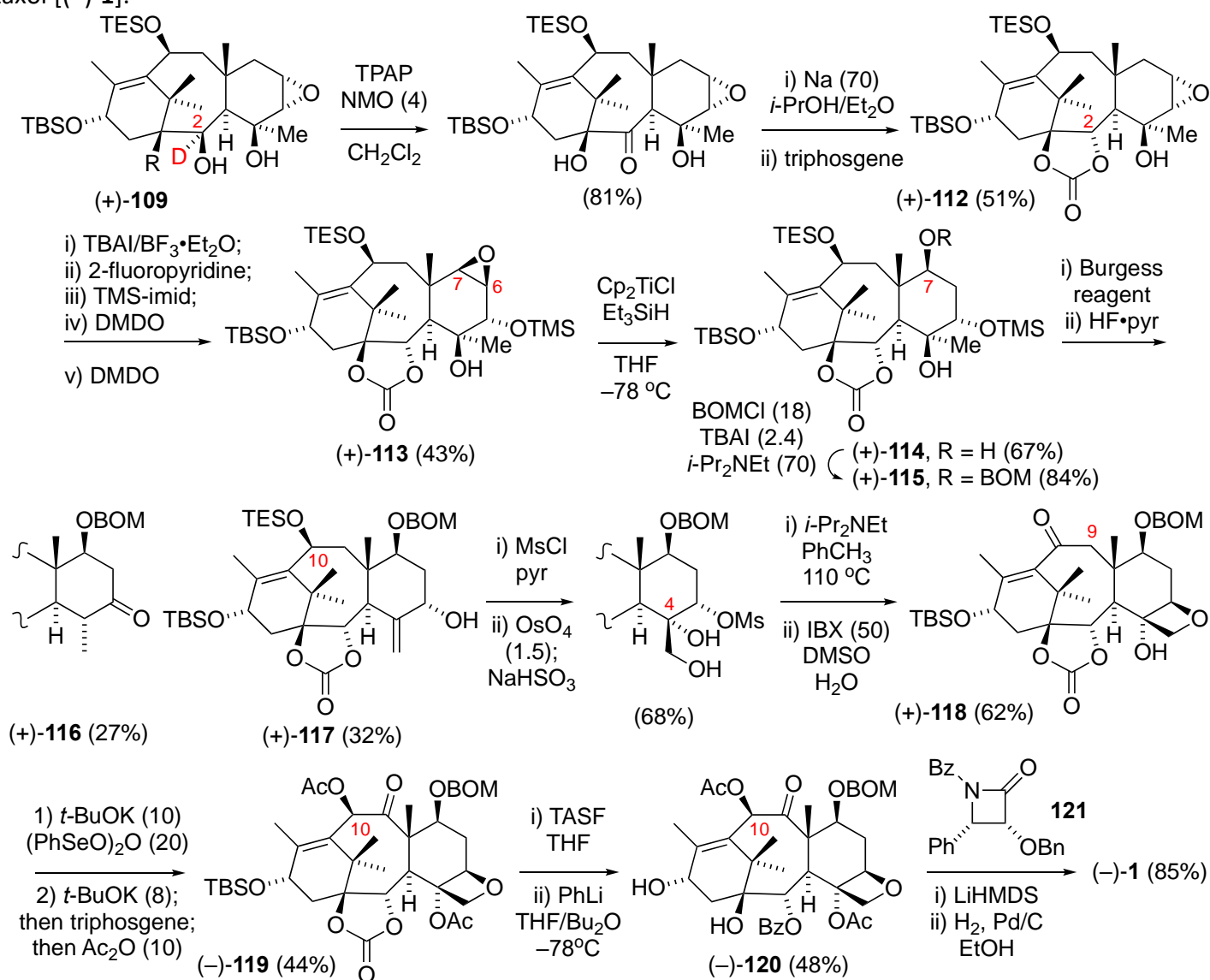
Scheme 19. Baran taxol synthesis end-game
