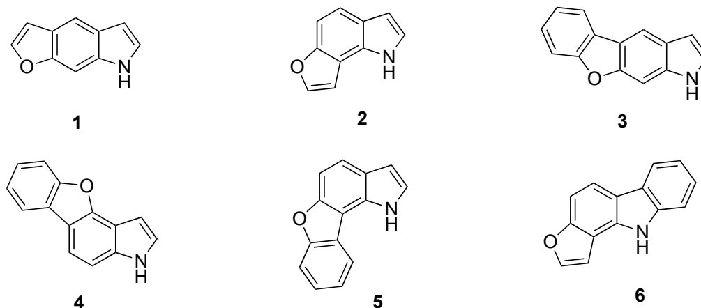
Figure 1. Some tri- and tetra-furanoindole structures 1-6 .
