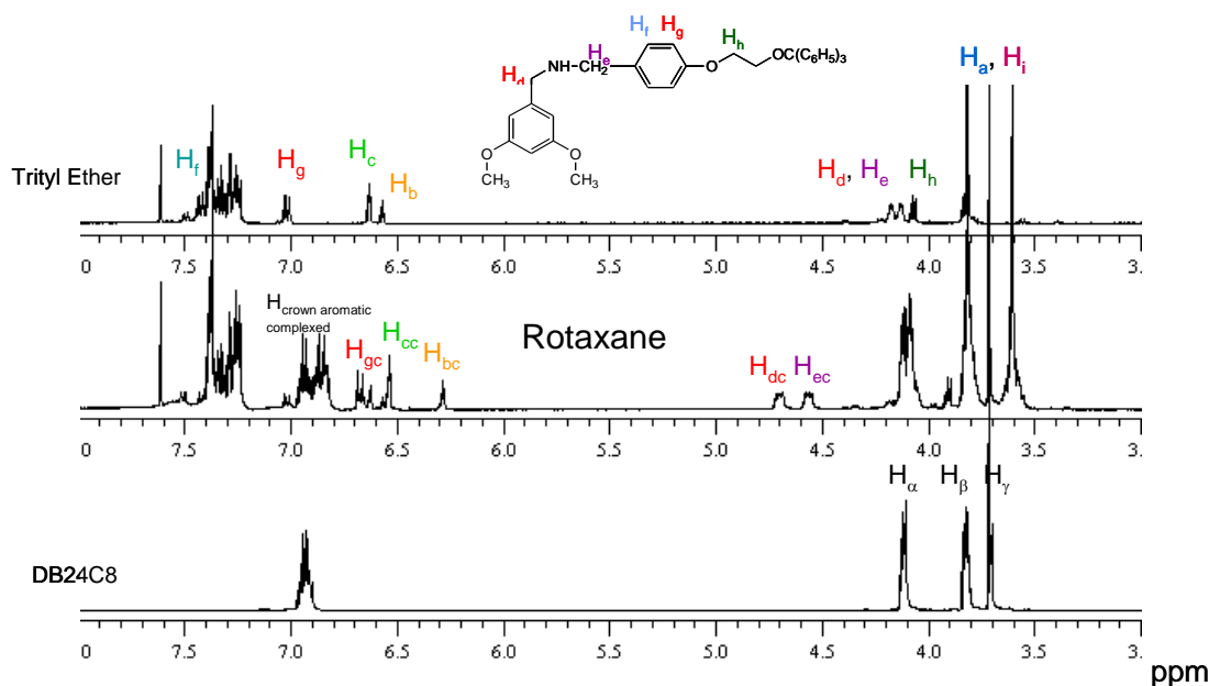
Figure 10. Stacked ^1\text{H} NMR spectra ( \text{CD}_3\text{CN} , 400 MHz, ambient T) of trityl ether 13 , rotaxane 14 , and DB24C
