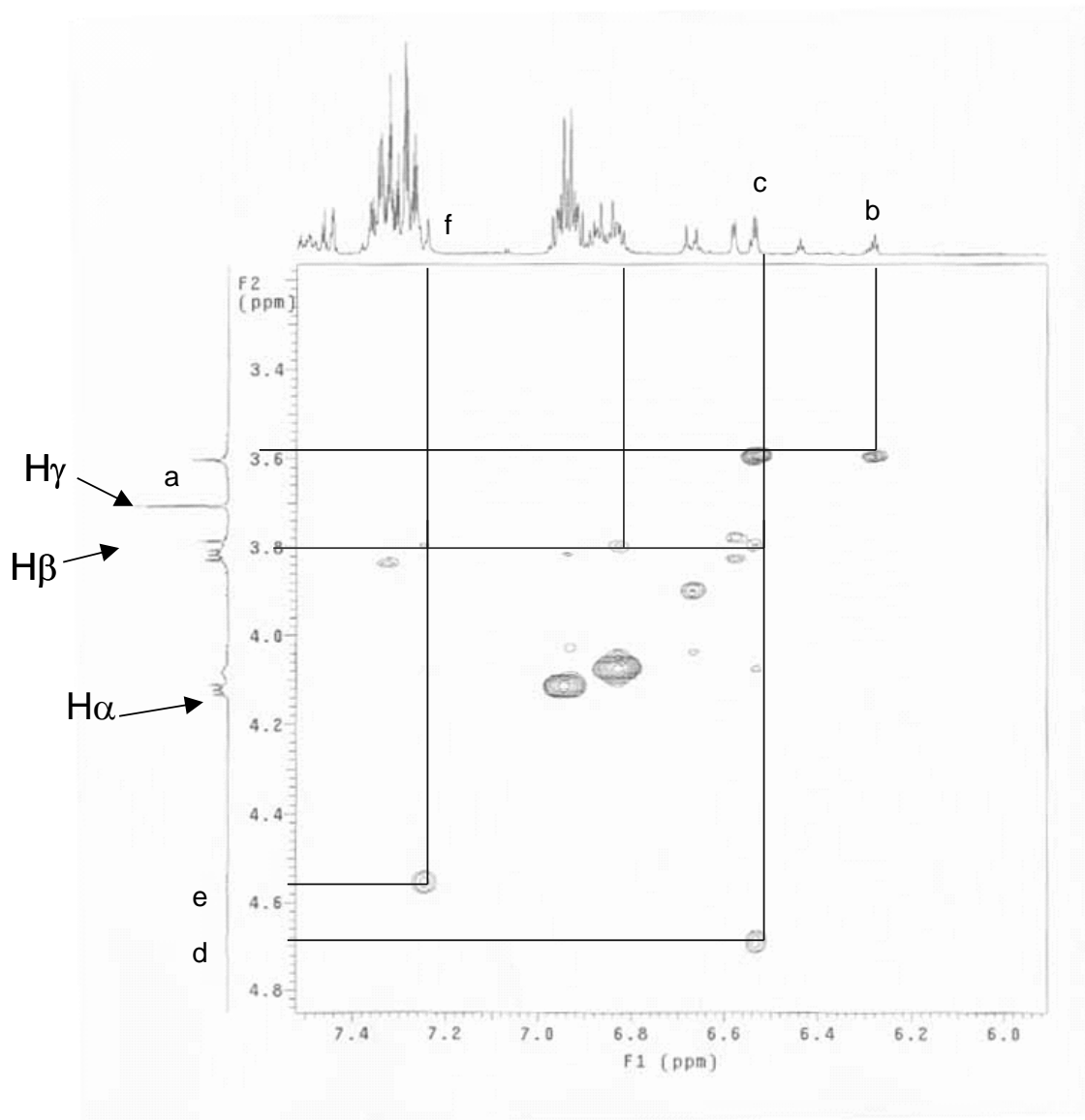
Figure 11. Partial NOESY ^1\text{H} NMR spectrum of rotaxane 14 (2/3 \text{CD}_3\text{CN}/\text{CDCl}_3 , 400 MHz, 23 ^\circ\text{C} ).
