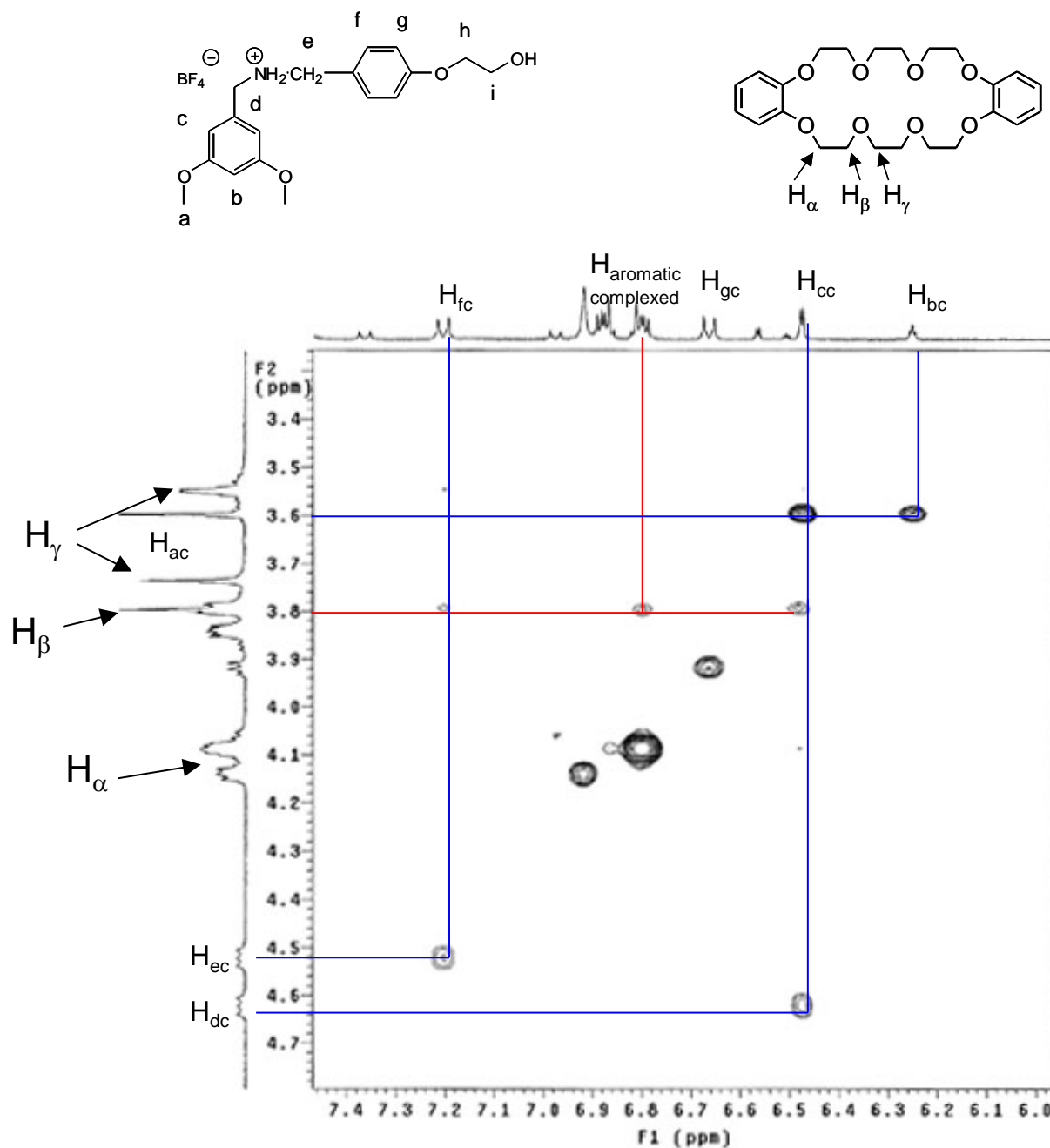
Figure 5. Partial ^1\text{H} NMR NOESY spectrum of \text{BF}_4 salt 5a + DB24C8 (10 mM each, \text{CD}_3\text{CN} ).
