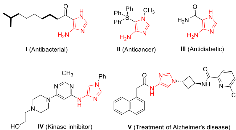
Figure 1. Selected drug molecules containing the 4-aminoimidazole moiety.
