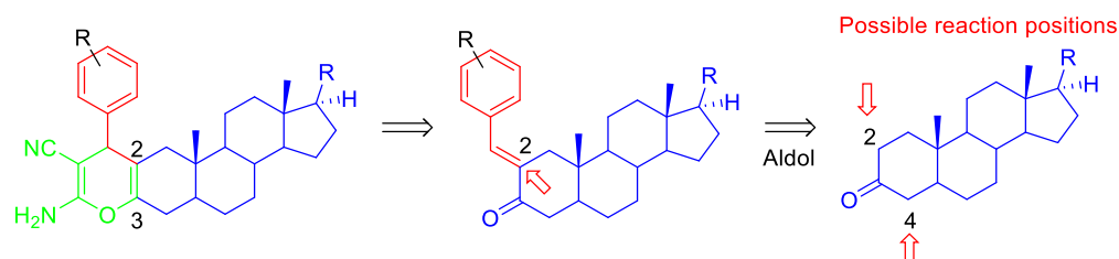
Figure 4. Retrosynthetic analysis of the two-step synthetic methodology. Regioselective functionalization of C-2:C-3 A-ring side of cholestane.
