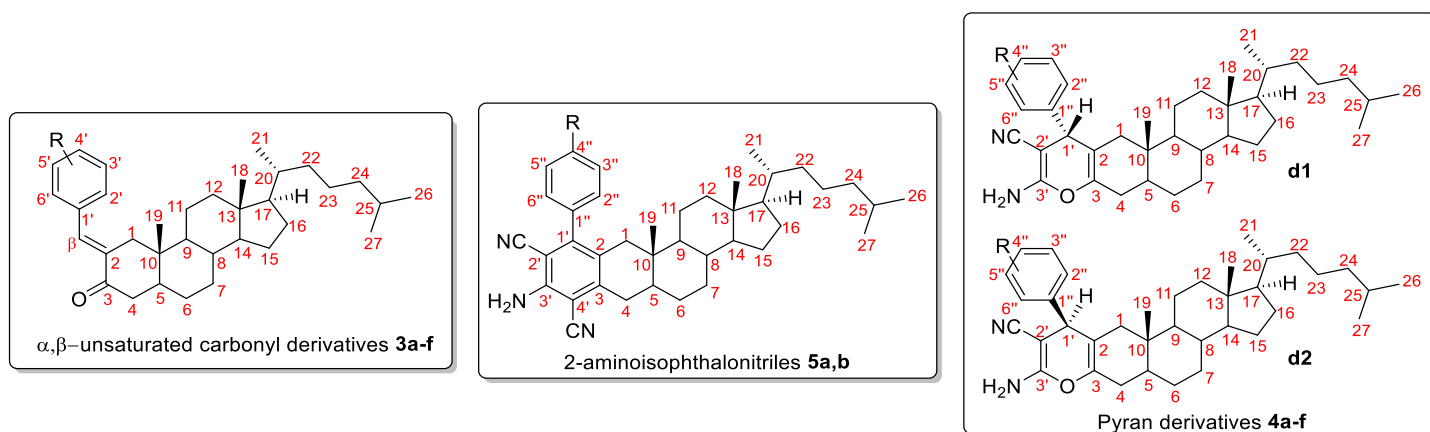
Figure 5. Arbitrary numbering of compounds 3a-f , 4a-f and 5a,b for NMR analysis and characterization.
