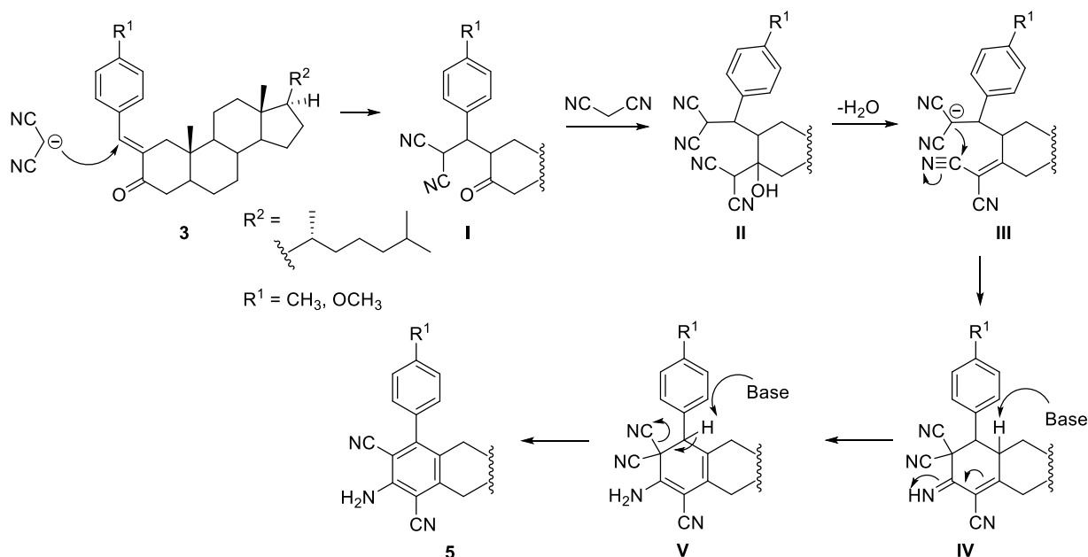
Scheme 2. Plausible mechanism for the formation of 2-aminoisophthalonitrile derivatives 5b,c .
