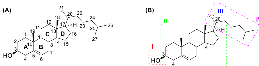
Figure 1. (A) Numbering and ring-labeling convention in cholesterol; (B) four domains of cholesterol.
