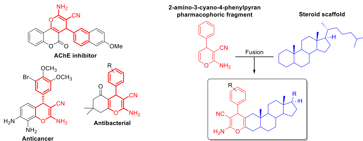
Figure 3. A-ring fused pyran derivatives.
