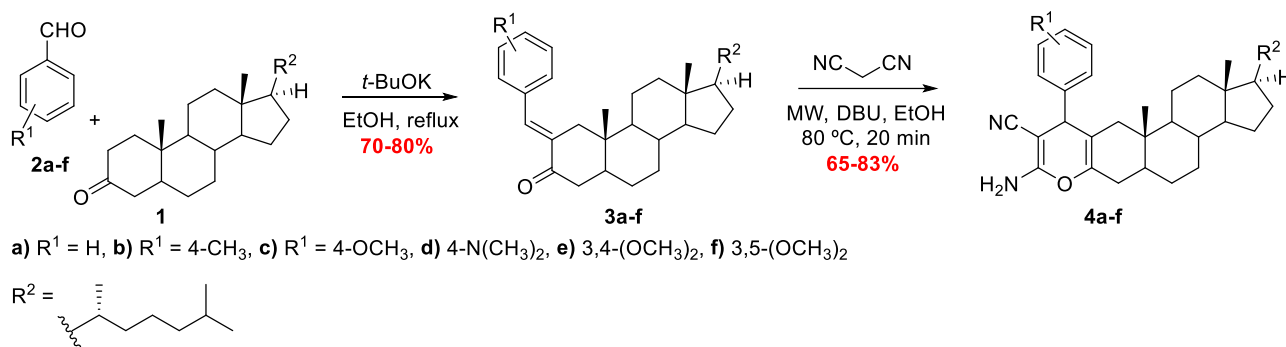
Scheme 1. Synthetic strategy for the two-step preparation of pyran-fused cholesterol derivatives 4a-f .
