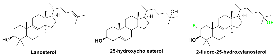
Figure 2. Chemical structures of lanosterol, 25-hydroxycholesterol, and 2-fluoro-25-hydroxylanosterol.
