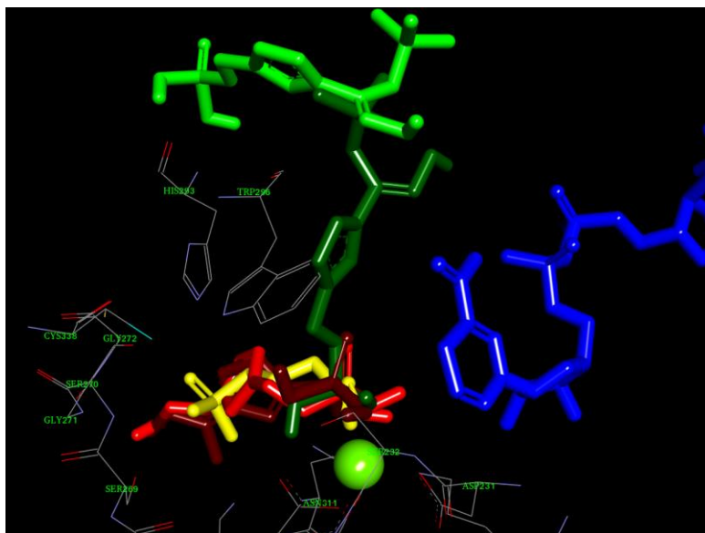
Figure 3. Best binding pose of 3a (red) and 3b (brown) to the PfDXR structure 3AU9_A 44 showing reverse binding (with phosphate close to the Mg 2+ cation) relative to fosmidomycin 1 yellow. 3c binds externally (light green) with higher energy poses penetrating the active site (dark green). The cofactor is shown in blue and the Mg cation as a sphere.
