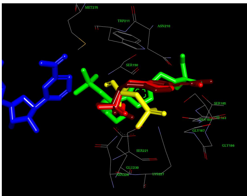
Figure 4. Best binding pose of 3a (red) and 3b (brown) to the EcDXR structure 2EGH_B 24 showing “reverse” binding (with phosphate close to the Mg cation). 3c (green) interacts with the Mg (behind) in a similar manner to fosmidomycin 1 (yellow). The cofactor is shown in blue and the Mg 2+ cation (behind) as a green sphere.
