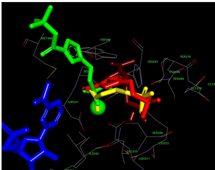
Figure 5. Best binding pose of 10a (red), 10b (brown) and 10c (green) to the PfDXR structure 3AU9_B. 44 10a and 10b , together with DOXP (not shown) bind in an arrangement similar to fosmidomycin 1 (yellow). 10c penetrates through to the active site. The cofactor is shown in blue and the Mg^{2+} cation as a sphere.
