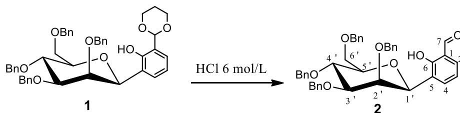
Scheme 2. Cleavage of dioxane ring in compound 1 to generate the compound 2
