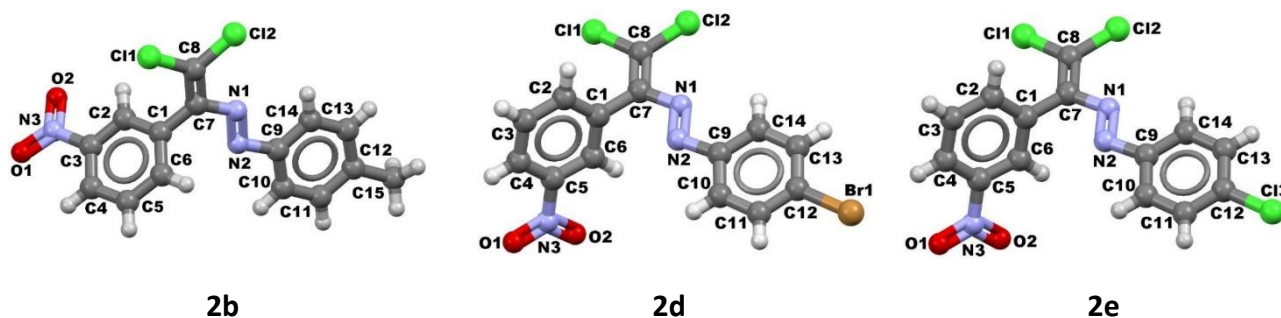
Fig. 1. Molecular structures of 2b , 2d and 2e (50% ellipsoids) along with the atomic numbering schemes.
