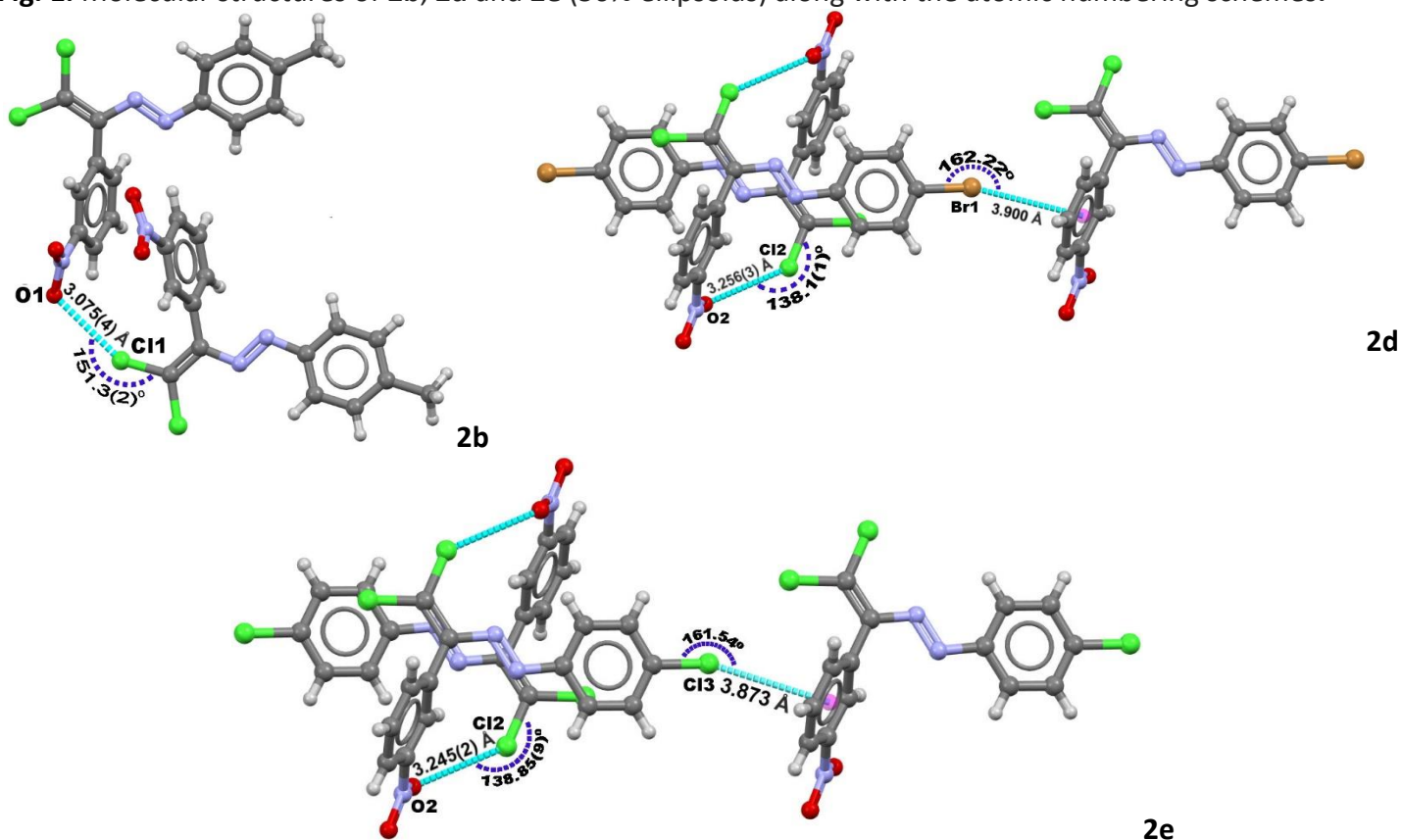
Fig. 2. Intermolecular halogen bonds in 2b , 2d and 2e (shown as dashed light blue line)
