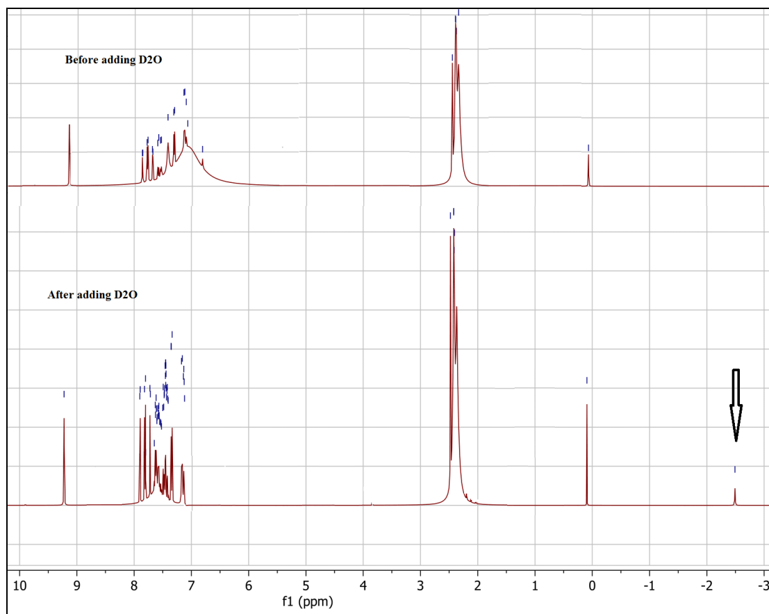
Figure 1. ^1\text{H-NMR} spectrum of the free base porphyrin ( 3a ) in \text{CDCl}_3 after and before adding \text{D}_2\text{O} and the disappearance of the signal for exchangeable inner 2NH at about -2.52 ppm.
