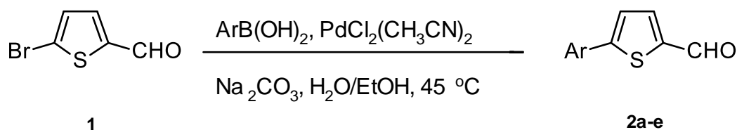
Scheme 1. Synthesis of 5-arylthienyl-2-carbaldehyde ( 2a-e ) using SMC reaction
