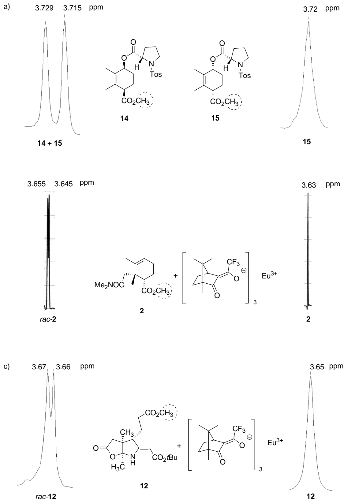
Figure 2. (a) Determination of enantiomeric excess of cis -alcohol 5 by ^1\text{H} NMR of its diastereomeric tosyl proline derivatives 14 and 15 (methyl ester signals). (b) Determination of enantiomeric purity of rearrangement product 2 by ^1\text{H} NMR shift experiment with chiral \text{Eu}(\text{TFC})_3 (methyl ester signals). (c) Determination of enantiomeric purity of building block 12 by ^1\text{H} NMR shift experiment with chiral \text{Eu}(\text{TFC})_3 (methyl ester signals).
