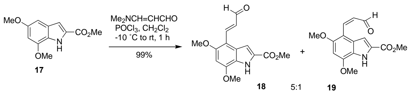
Scheme 5. Formation of 4-indolylpropenals 18 and 19 .
