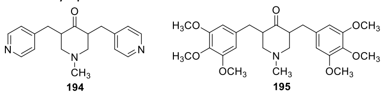
Figure 17. Structures of anticancer MACs 194-195 .
