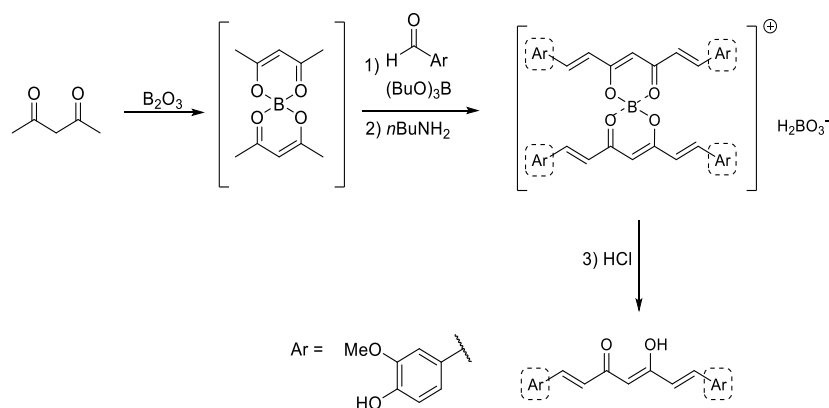
Figure 3. General synthetic route to curcumin
