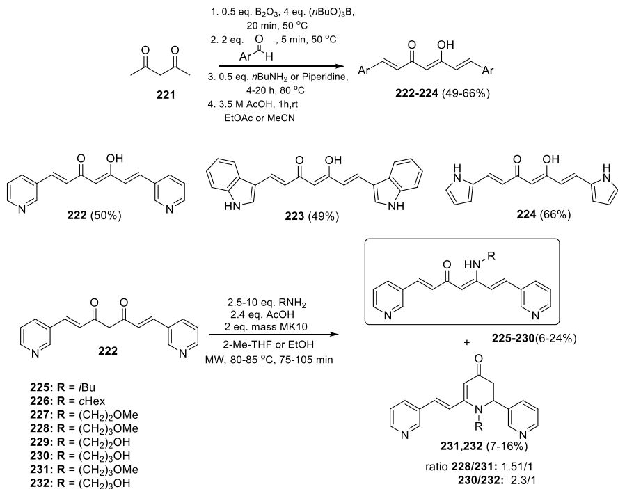
Scheme 15. Synthesis of \beta -enaminones 222-232 .
