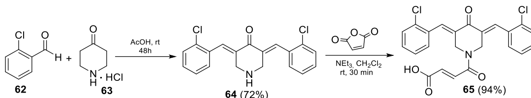
Scheme 12. Synthetic approach towards 3,5-bis(2-chlorobenzylidene)-4-piperidones 64 and synthesis of N -acryl derivatives of 3,5-bis(2-chlorobenzylidene)-4-piperidone 65 .
