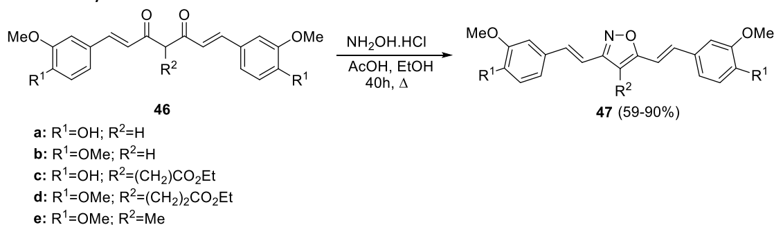
Scheme 6. Synthesis of isoxazole curcuminoids via Paal-Knorr chemistry 47 .
