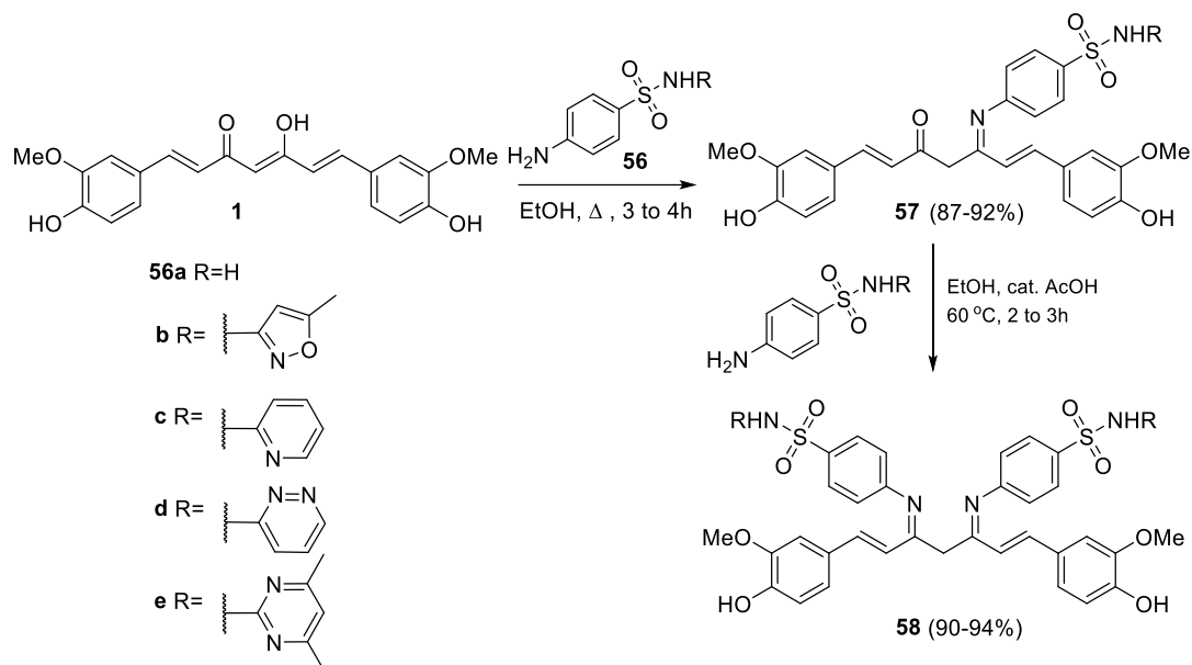
Scheme 11. Synthesis of new derivatives of curcumin containing sulfonamides.
