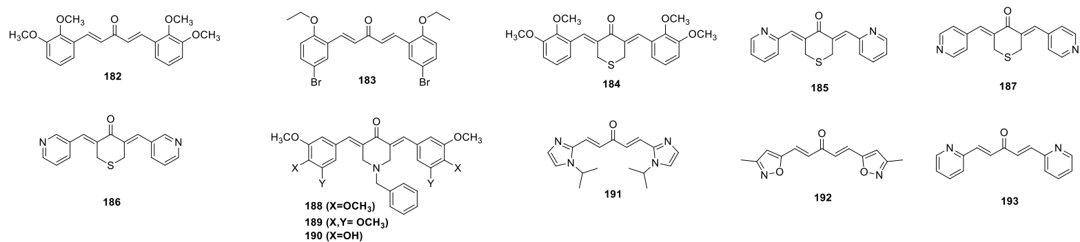
Figure 16. Structures of anticancer MACs 182-193.
