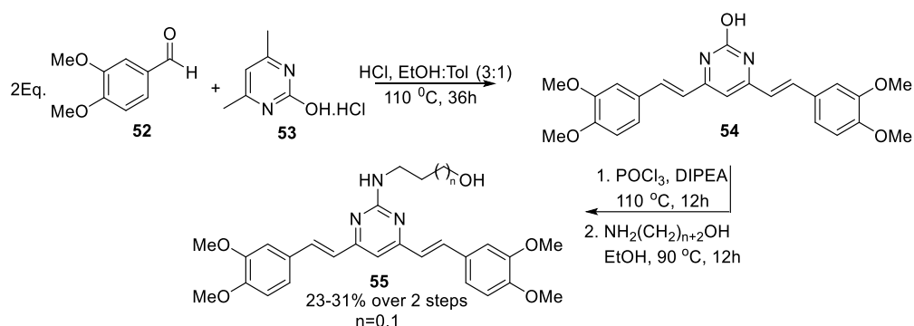
Scheme 10. Synthesis of pyrimidine-substituted curcumin analogs 55 .
