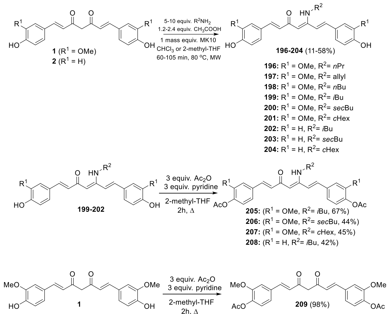
Scheme 13. Synthesis of \beta -enaminones 196-208 and bis-acetylated curcumin 209 .
