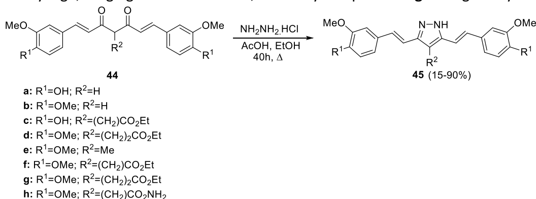
Scheme 5. Knorr pyrazole synthesis of pyrazole curcuminoids 45 .
