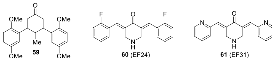
Figure 8. Monocarbonyl curcuminoids 59-61 . 163,164,204,207
