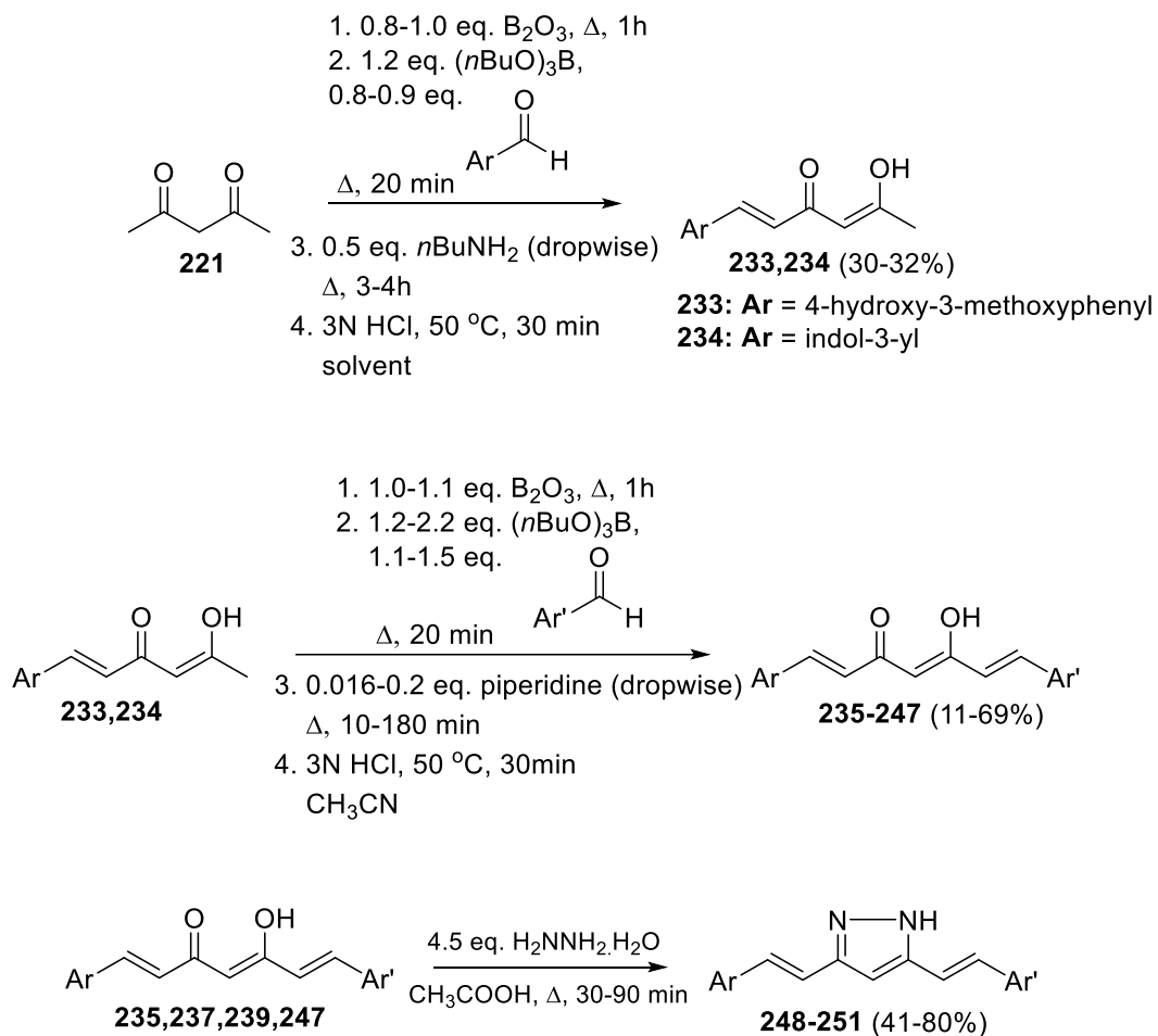
Scheme 16. Synthesis of \beta -enaminones 235-251 .
