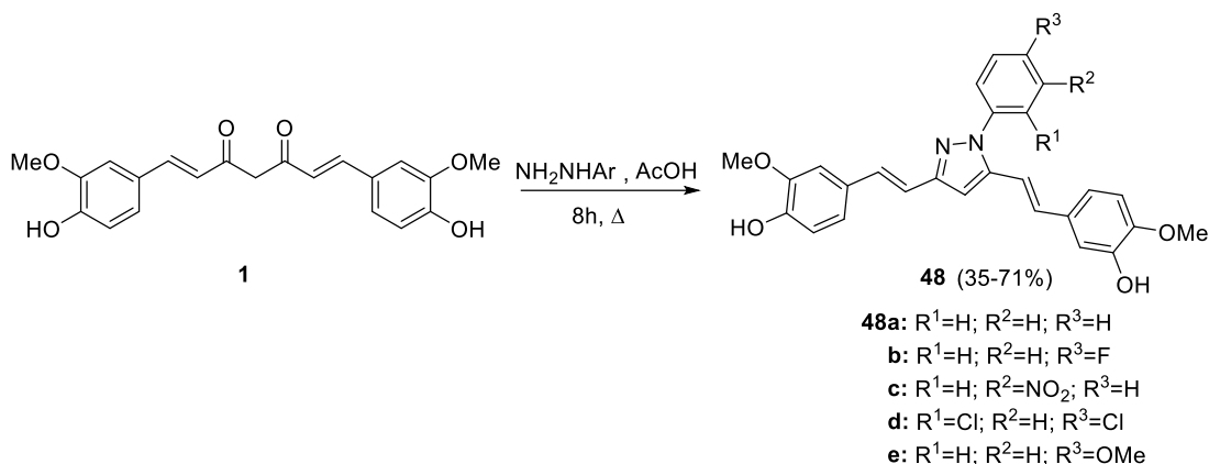
Scheme 7. Synthesis of N -arylpirazole analogs 48 .
