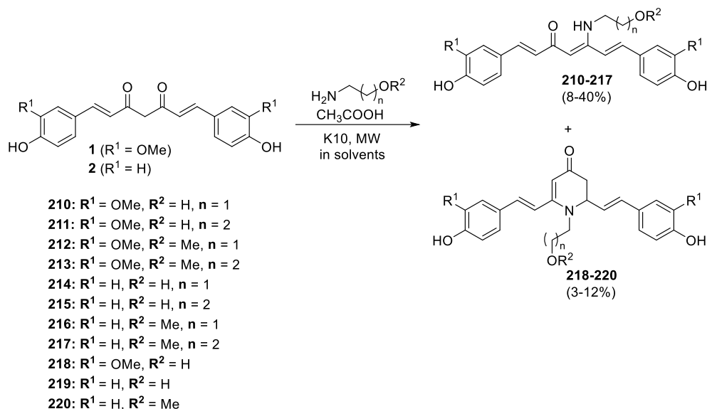
Scheme 14. Synthesis of \beta -enaminones 210-220 .
