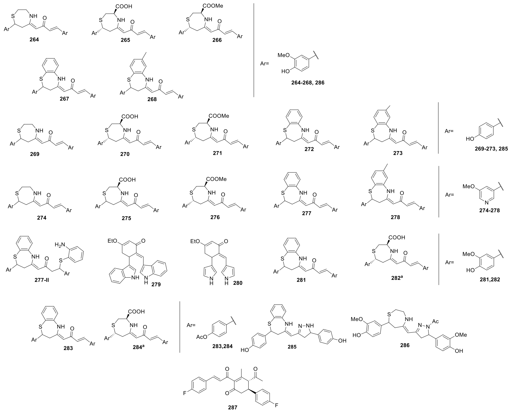
Figure 19. Structures of curcuminoids 264-287.
