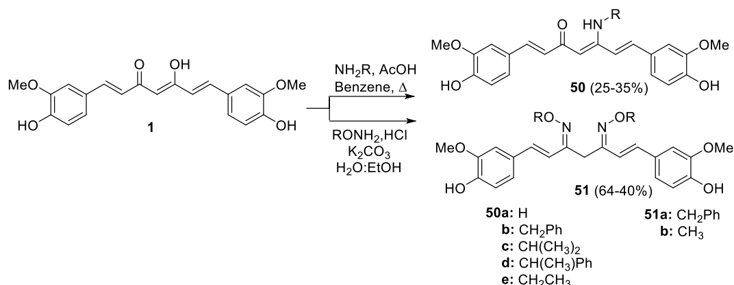
Scheme 9. Synthesis of mono/di-β-enaminone analogs 50 and 51 .
