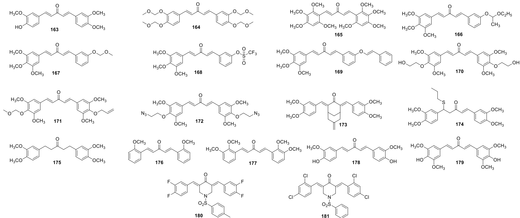
Figure 15. Structures of anticancer MACs 163-181.
