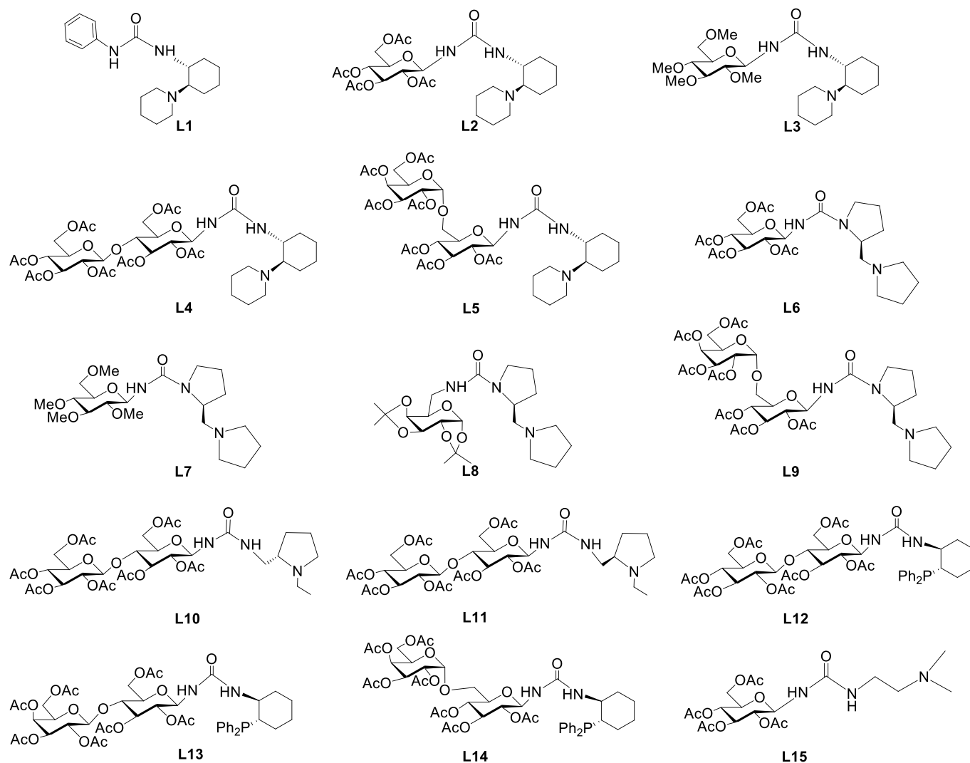
Figure 1. Organocatalysts screening.
