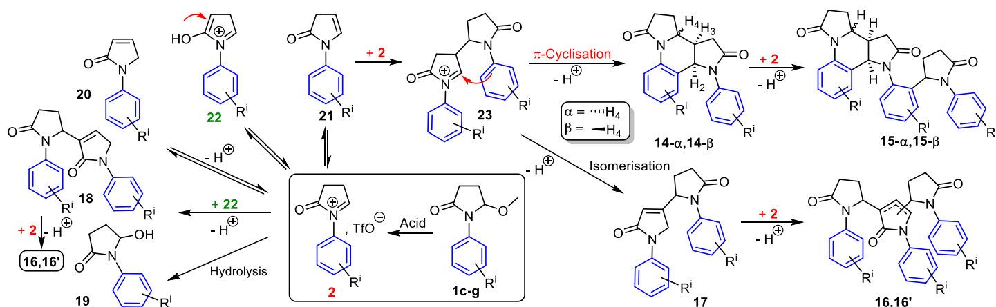
Scheme 9. Plausible mechanism for the formation of 14-20 from pterolactams 1c-g ( R^i are substituents).
