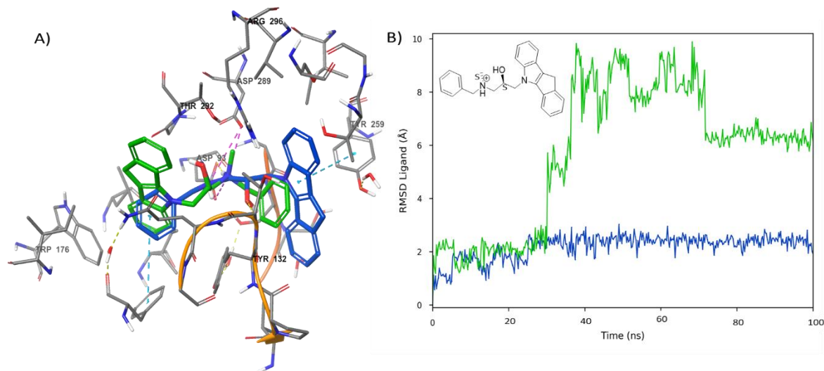
Figure 6. Overlaid docking poses of the two suggested binding poses of an enantiomer of 20 (S,S). Pose A (blue) has hydrogen bonding to the backbone nitrogen of Thr133 (shown in yellow), along with ionic interaction with Asp289 and Asp93. A \pi - \pi edge-to-face interaction is also present with Tyr259. Pose B (green) has the \pi - \pi interaction with Phe169, hydrogen bonding to Asp93, and ionic interactions with Asp93 and Asp289. For clarity, selected residues of the binding pocket have been hidden. A plot of the ligands RMSD during the course of the 100 ns MD simulation is shown for pose A and pose B in blue and green, respectively. The ligand RMSD is indicative of how stable the ligand is with respect to the protein's backbone.
