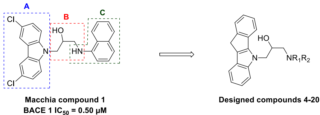
Figure 4. Design strategy of target compounds 4-20 .
