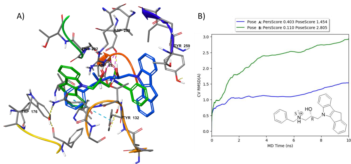
Figure 5. A) Overlaid docking pose of the two suggested binding poses of the ( S,R ) enantiomer of 20 from the induced fit docking. Pose A (blue) contains a hydrogen bond to Asp289 (shown in yellow), along with ionic interactions with Asp289 and Asp93 from the protonated tertiary nitrogen (shown in pink). Pose B (green) has the same ionic interactions with Asp289 and Asp93 as pose A, while \pi - \pi edge-to-face stacking is noted between Tyr132 and the tetracyclic ring. For clarity, selected residues of the binding pocket have been hidden. B) A plot of the ligands RMSD, averaged over the course of seven metadynamics simulations, with each simulation being 10 ns.
