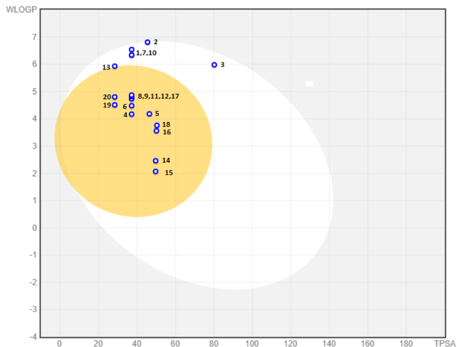
Figure 10. Boiled egg plot of WLogP vs. TPSA, yellow indicates BBB-permeant, white indicates gastrointestinal permeant, blue indicates P-glycoprotein +.
