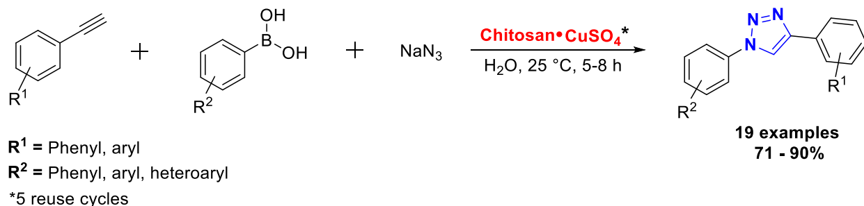
Scheme 41. Use of arylboronic acids in the multicomponent synthesis of 1H-1,2,3-triazole derivatives. 258
