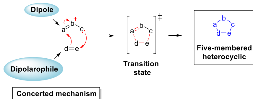
Scheme 7. Cycloaddition mechanism proposed by Huisgen. Adapted from Bräse, 2010. 55
