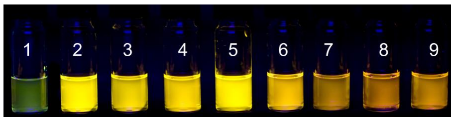
Figure 3. Emission colors of derivative 5 in various solvents; \lambda_{\text{ex}} = 366 \text{ nm} . 1: H 2 O, 2: 2-PrOH, 3: AcOH, 4: EtOH, 5: 1-BuOH, 6: THF, 7: MeOH, 8: MeCN, 9: DMSO.
