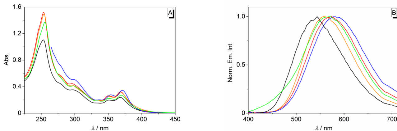
Figure 2. Absorption ( c = 20 \mu\text{M} ) (A) and normalized emission spectra (Abs. = 0.10 at \lambda_{\text{ex}} = 365 \text{ nm} ) (B) of derivative 5 in H 2 O (black), MeOH (red), 2-PrOH (orange), THF (green), and DMSO (blue).
