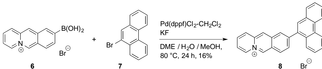
Scheme 1. Synthesis of 8-(phenanthren-9-yl)benzo[ c ]quinolizinium tetrafluoroborate ( 5 ). Reagents and reaction conditions: i) Fe, aq. HCl (37%), aq. NH 4 Cl (25%), EtOH, 65 °C, 2 h; ii) NaBF 4 , H 2 O, 62%; iii) NaNO 2 , aq. HBr (24%), 0 °C, 10 min; iv) CuBr, aq. HBr (48%), rt, 1 h, 26%.
