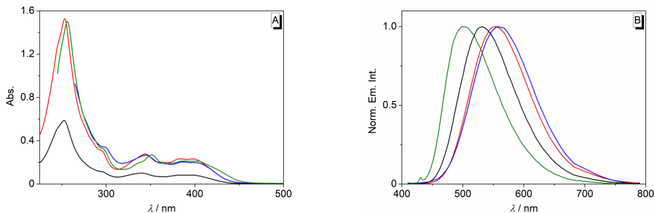
Figure 4. Absorption ( c = 20 \mu\text{M} ) (A) and normalized emission spectra (Abs. = 0.10 at \lambda_{\text{ex}} = 399 \text{ nm} ) (B) of derivative 8 in H 2 O (black), MeOH (red), CHCl 3 (olive), and DMSO (blue).
