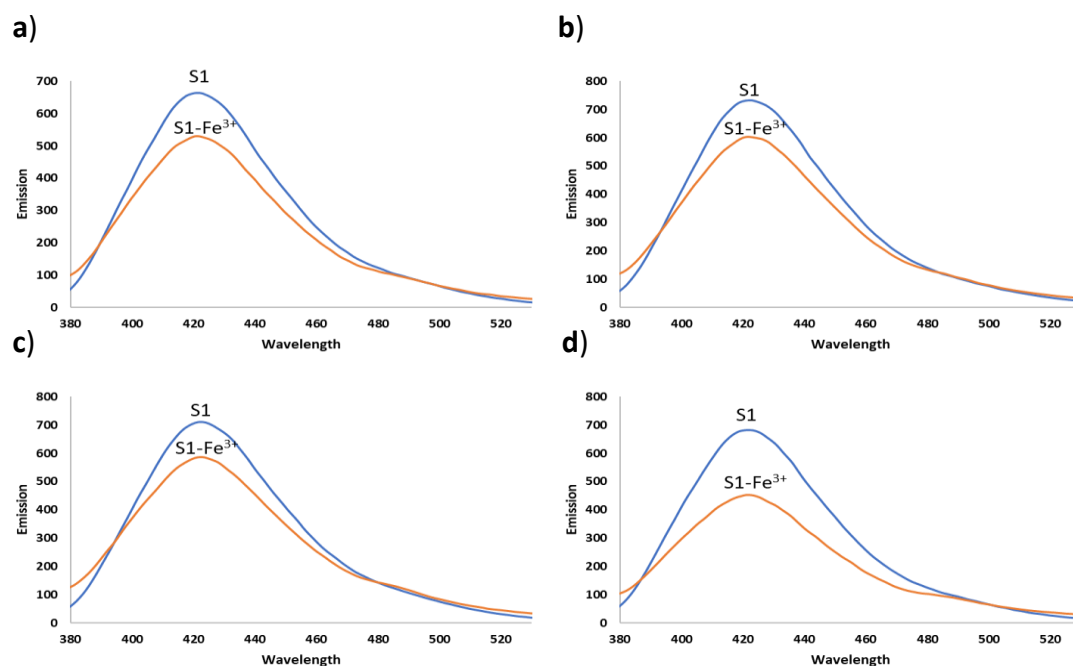
Figure 16. Effect of pH on S1 and \text{Fe}^{3+} quenching behavior at (a) original pH, (b) pH 4, (c) pH 5, and (d) pH 10.
