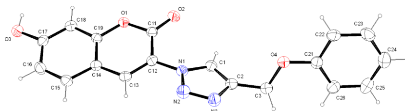
Figure 2. X-ray crystal structures of triazolyl-coumarin derivatives S1 (a) and S2 (b).
