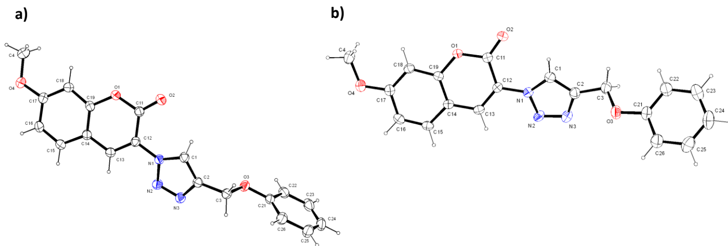
Figure 10. a) Crystal X-Ray diffraction of S1 before complexation; b) after interaction with \text{Fe}^{3+} at lower concentrations.
