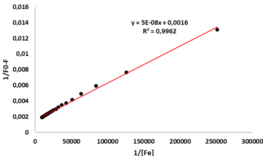
Figure 13. Benesi-Hildebrand plot of S1 with Fe^{3+} in water.
