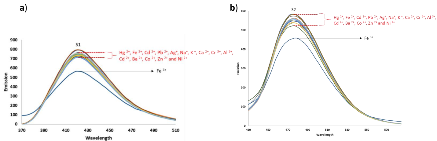
Figure 5. Fluorescent responses of (a) S1 and (b) S2 with selected metal cations in water. Excitation: 340 nm.
