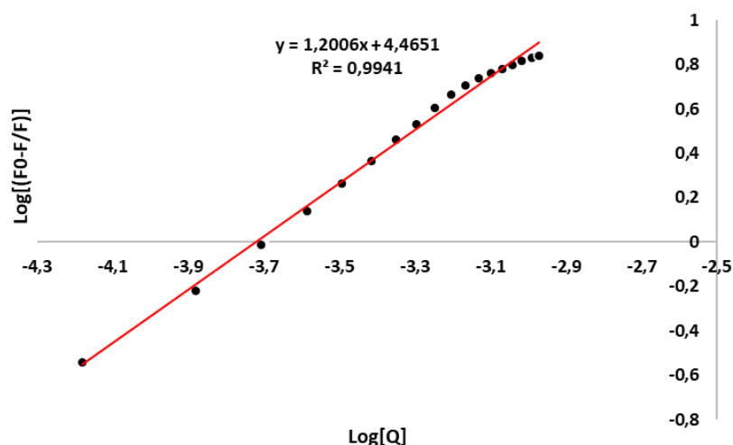
Figure 23. Logarithmic plot of the fluorescence quenching of S1 with various amounts of Fe 3+ in excitation wavelength of 340 nm.
