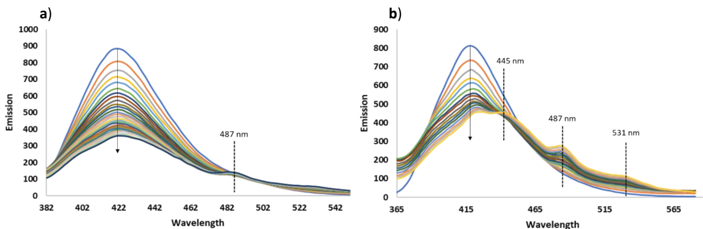
Figure 8. Changes in the fluorescence spectrum of S1 in a) water and b) acetonitrile upon addition of Fe 3+ ions. Excitation: 340nm. Titration conducted in triplicate.
