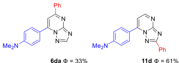
Figure 5. Quantum yields of 6da and 11d .
