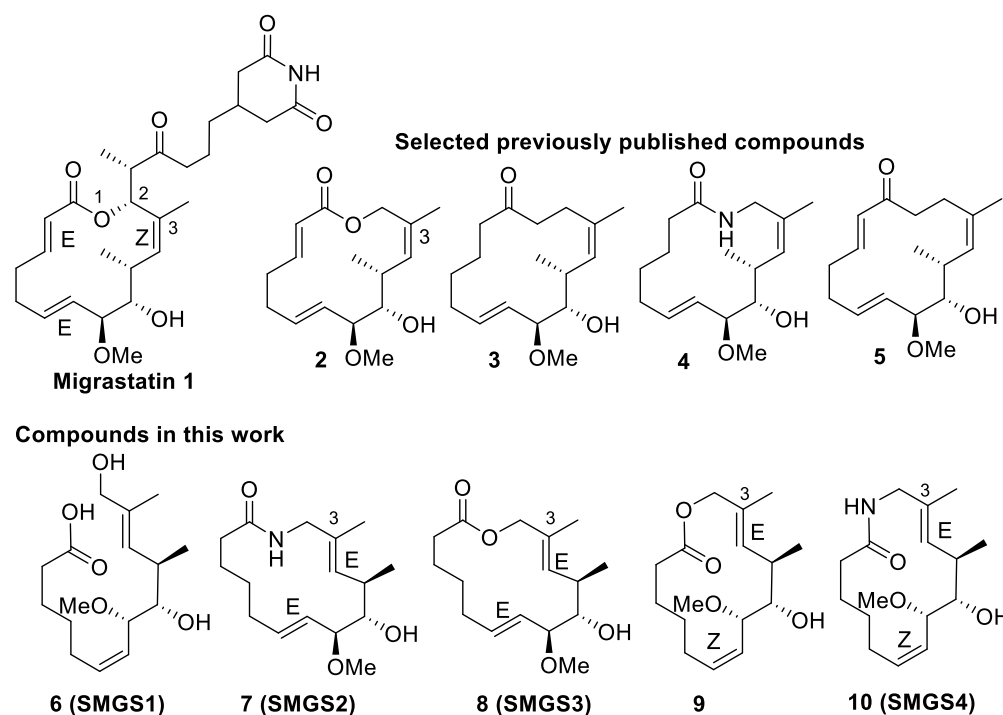
Scheme 1: Structures of compounds 1-10 .
