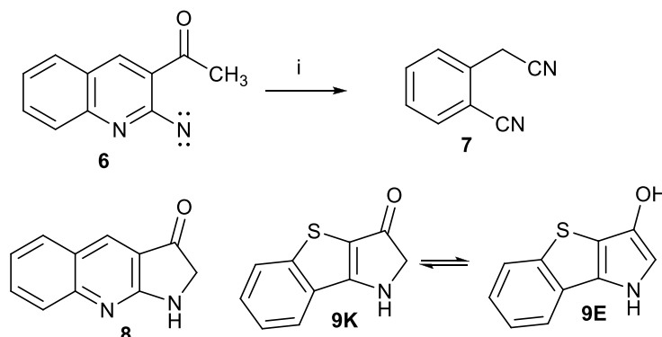
Scheme 2. Reagents and conditions: (i) FVP 600 °C
