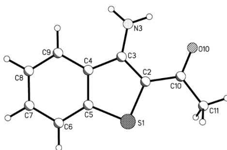
Figure 1. Plot of one of the molecules of 10 showing the crystallographic numbering scheme
