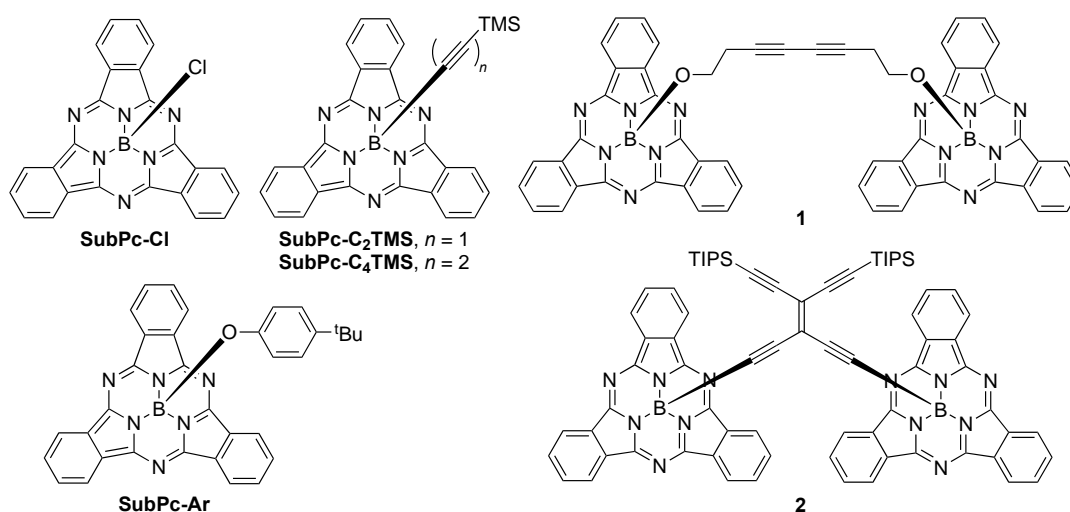
Figure 1. Known boron subphthalocyanine (SubPc) monomers and dimers.
