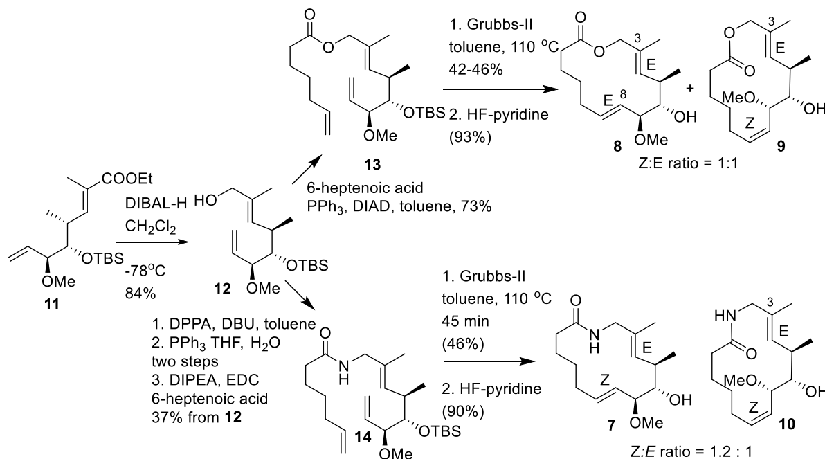
Scheme 2. Synthesis of 7-10
