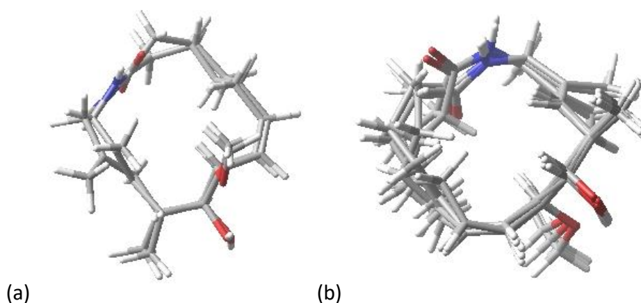
Figure 2. (a) Overlap of X-ray structure with lowest energy structure generated by conformational search in MacroModel is shown on the left. Overlay was generated by superimposing macrocyclic backbone atoms NH to C-10 (RMSD = 0.25) (b) Five superimposed isomers generated within 10 kJ/mol of global minimum as obtained from conformational search using MacroModel are shown on the right. Two of these five stereoisomers had a cis-amide conformation; the lowest energy conformer had the trans-amide.
