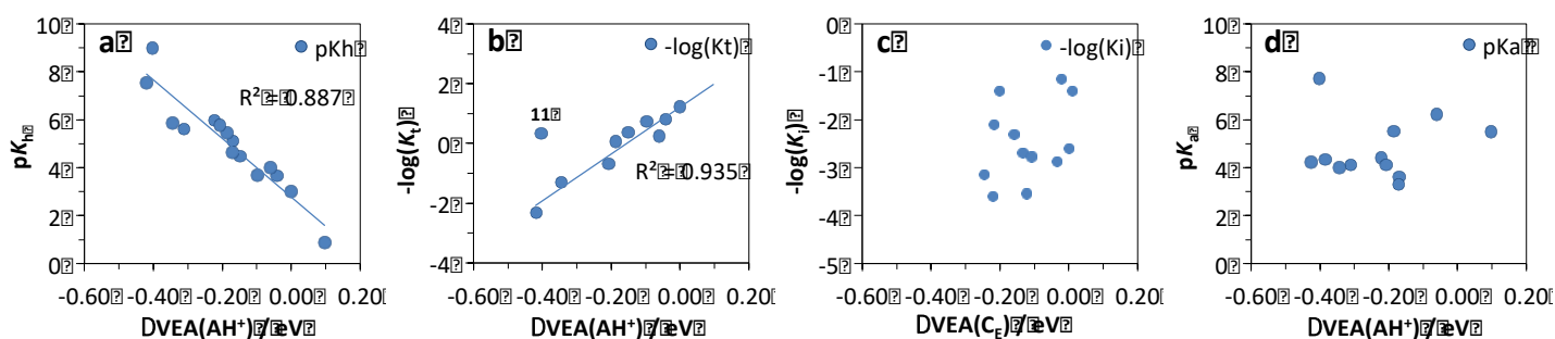
Figure 3. Representations of (a) pK_h and (b) -\log(K_t) as a function of the vertical electron affinity of AH^+ , (c) -\log(K_i) as a function of the VEA of the C_e form and (d) pK_a as a function of the VEA of the AH^+ form. The VEAs of the flavylum salt species were calculated at the mPW1PW91/6-31G(d) level of theory.
