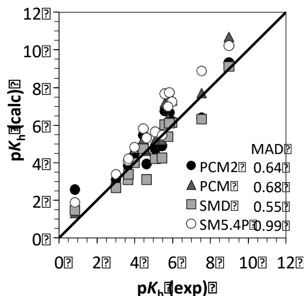
Figure 1. Calculated pK_h values for the flavylium salts studied and the respective mean absolute deviations (MAD) for the solvation models utilized. The straight line corresponds to pK_h calculated = pK_h experimental and is included to guide the eye.
