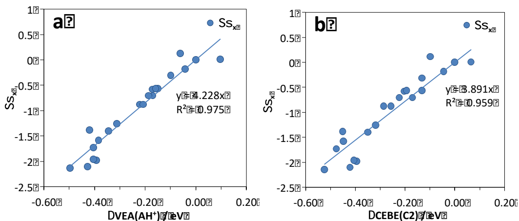
Figure 2. Correlation of the sum of the Hammett constants of substituents of flavylum cations with the: (a) vertical electron affinity and (b) core-electron binding energy of C2(1s) of the AH^+ form.
