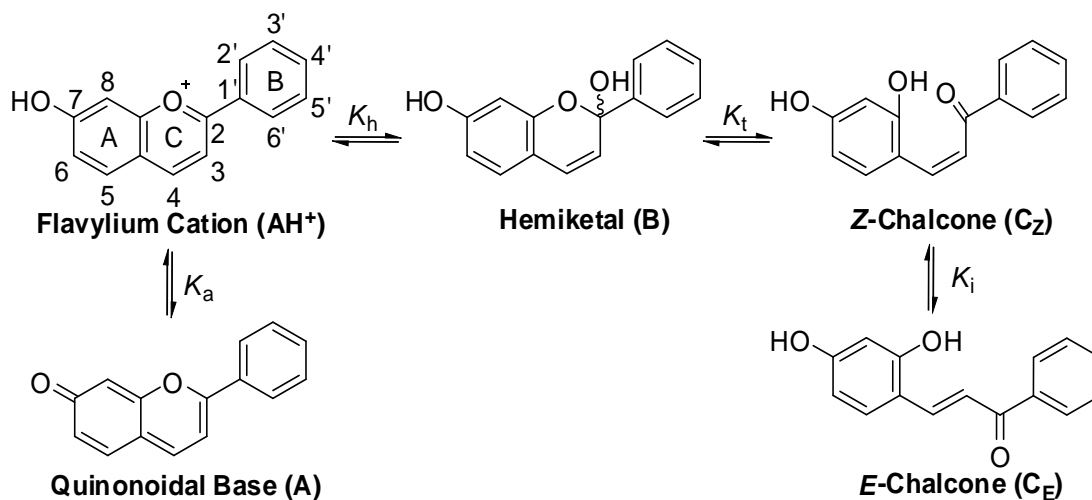
Scheme 1. Chemical transformations of hydroxyflavylum salts.
