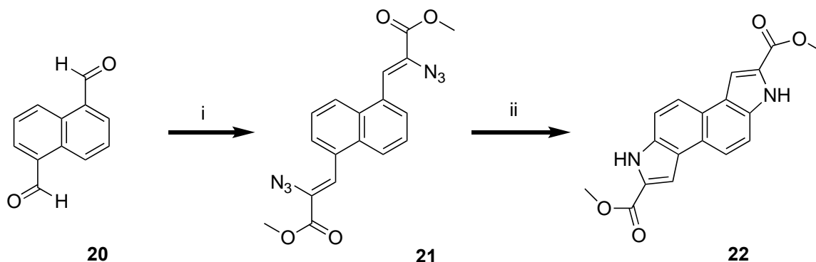
Scheme 3. Reagents and conditions: i: \text{N}_3\text{CH}_2\text{CO}_2\text{Me} , \text{NaOMe} , anhyd. \text{MeOH} <-10\text{ }^\circ\text{C} , 4 h, 67%, ii: xylene reflux, 6 h
