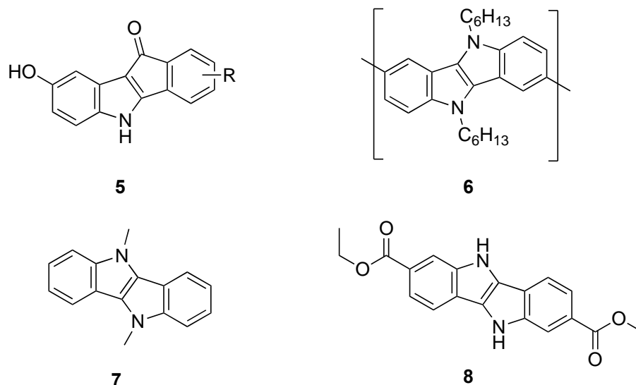
Figure 2. Biologically and photophysically important dihydroindoloindole systems
