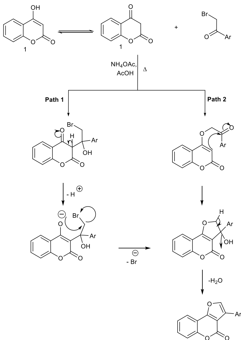
Scheme 2. Possible mechanism of 3-aryl-furo[3,2-c]coumarin derivatives.
