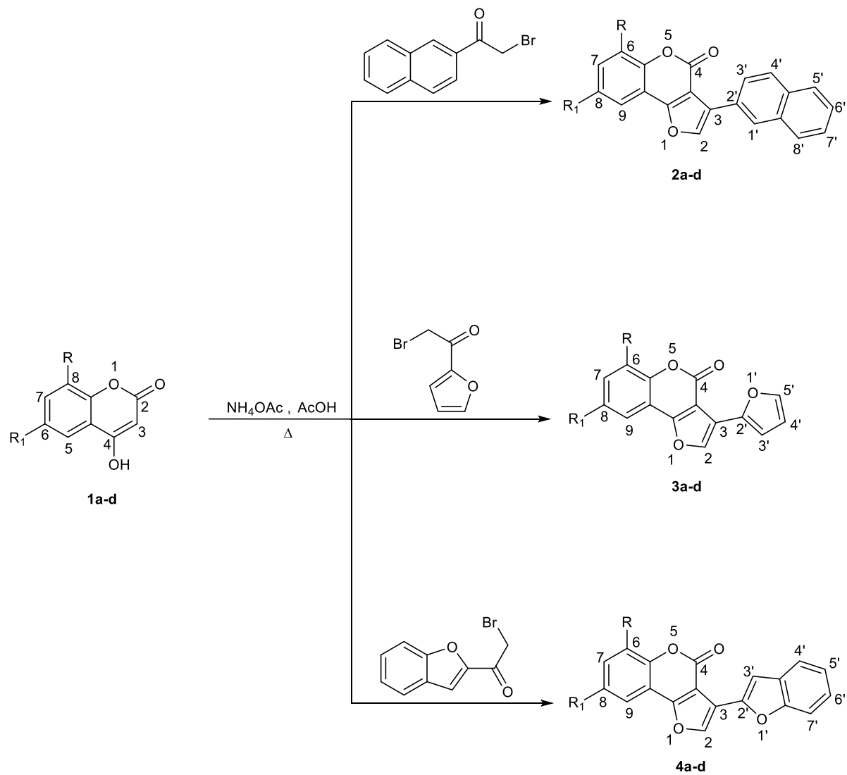
Scheme 1. 3-Aryl-furo[3,2-c]coumarins
