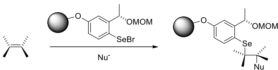
Scheme 11. Selenylation of olefins using immobilized selenium reagents. 50
