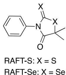
Figure 5. Cyclic RAFT agents containing sulfur or selenium atoms. 38
