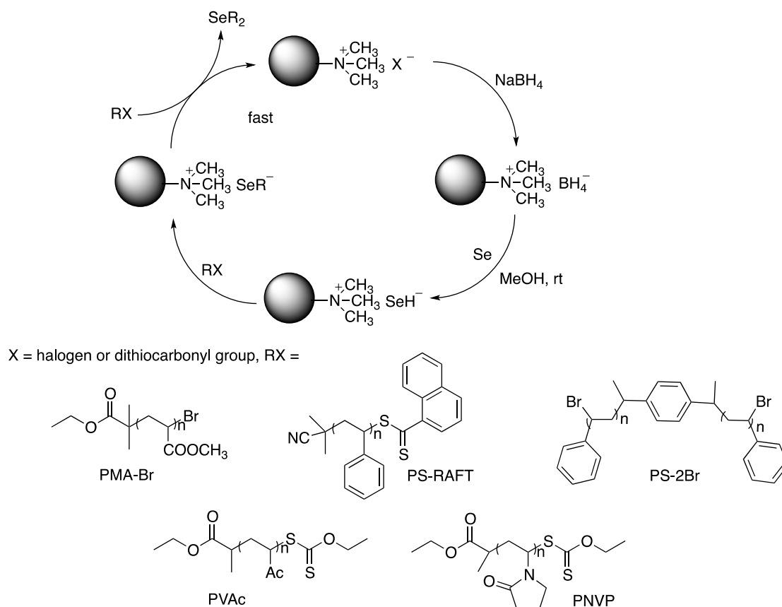
Scheme 8. The application of ion-exchange resin to the synthesis of selenium-containing polymers. 41
