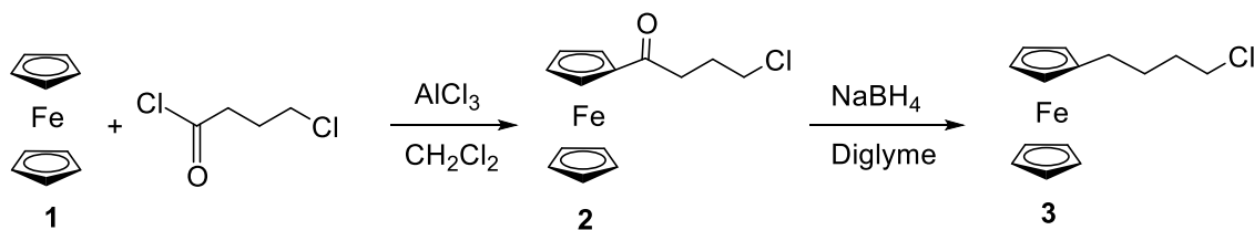
Scheme 1. Synthesis of 4-chlorobutylferrocene (3).
