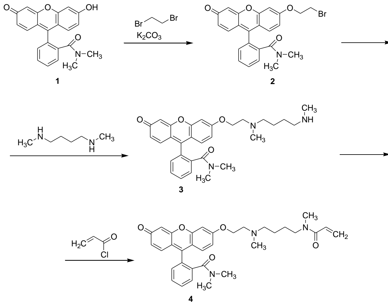
Scheme 4. Synthesis of new fluorescein compounds.
